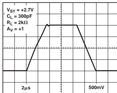
Figure 17. Large Signal Transient Response at +2.7 V
