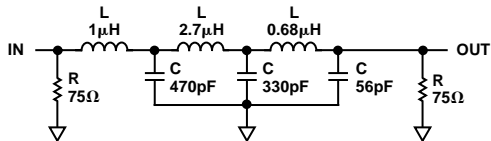
Figure 79. Output Filter
