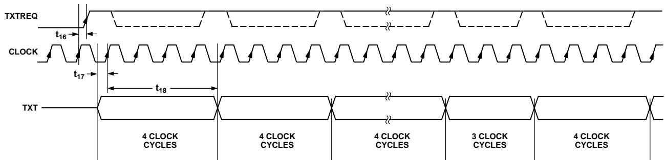
Figure 3. Teletext Timing Diagram
