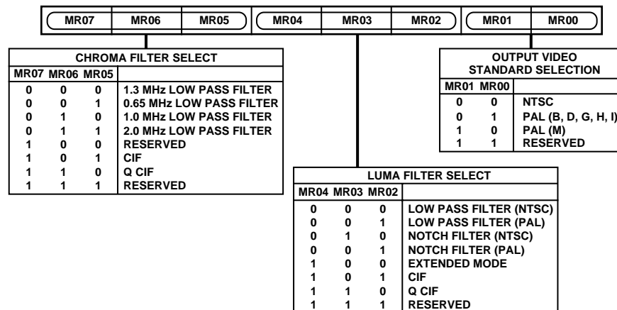
Figure 38. Mode Register 0
