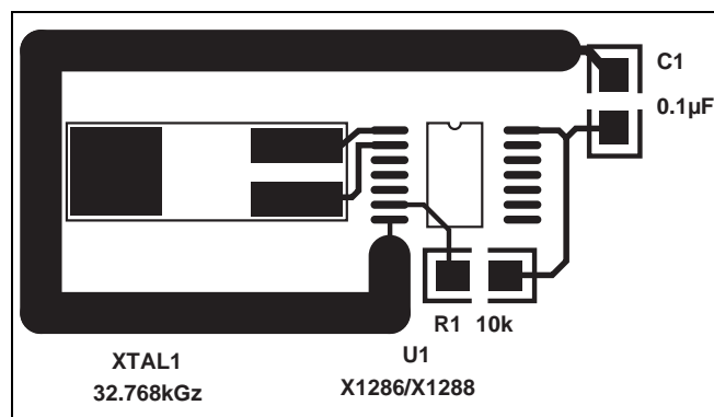
Figure 15. Suggested Layout for Intersil RTC in SO-8
