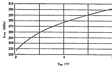
Note 11) Supply Voltage vs Oscillating Frequency
