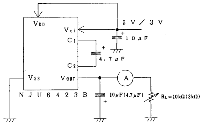
Note 10) Voltage Doubler Characteristics Measuring Circuit.
