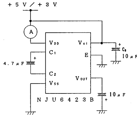
Note 10) Voltage Doubler Characteristics Measuring Circuit.
