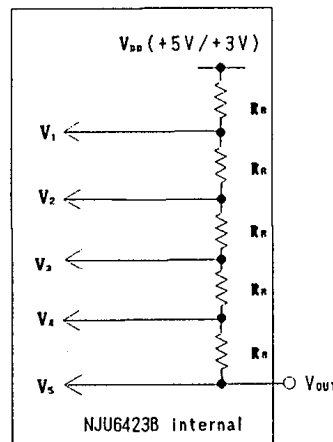
Internal Bleeder Resistance
