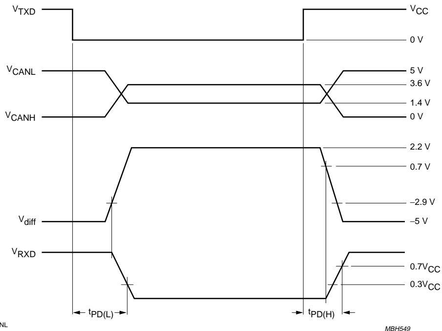
Fig.4 Timing diagram for dynamic characteristics.
