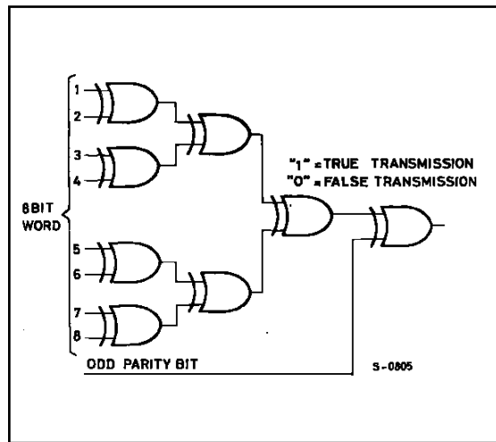
ODD-PARITY CHECKER (2 x HCC/HCF4030B).
