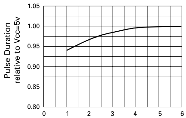
Normalized Output Pulse Duration v Supply Voltage
