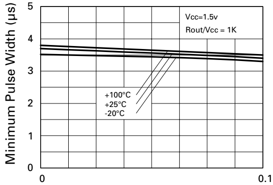
Minimum Pulse Width Required for Triggering
