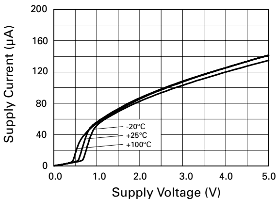
Supply Current v Supply Voltage
