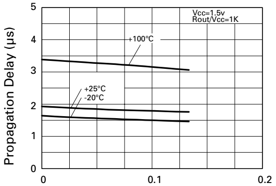
Output Propagation Delay
