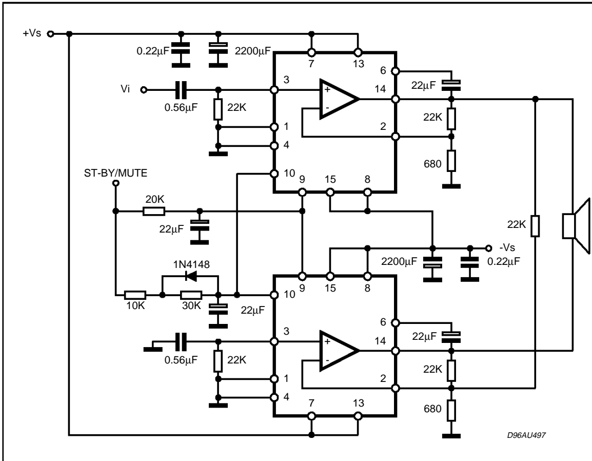
Figure 19: Bridge Application Circuit
