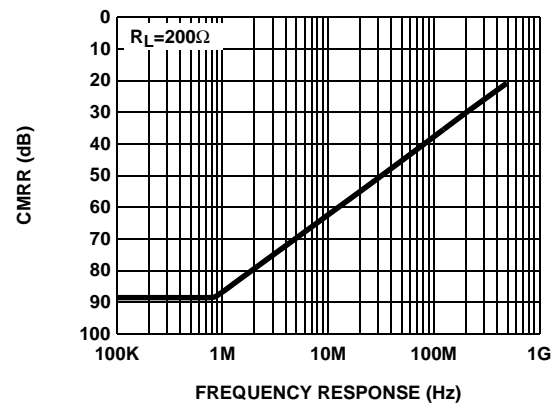
FIGURE 6. CMRR
