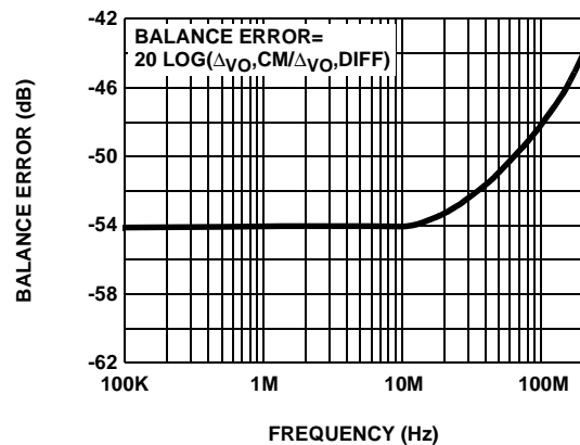
FIGURE 2. BALANCE ERROR
