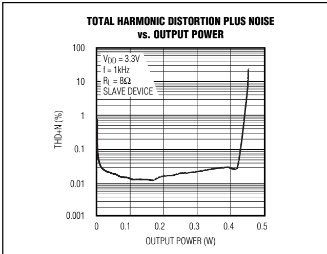
Figure 8. Master-Slave THD+N
