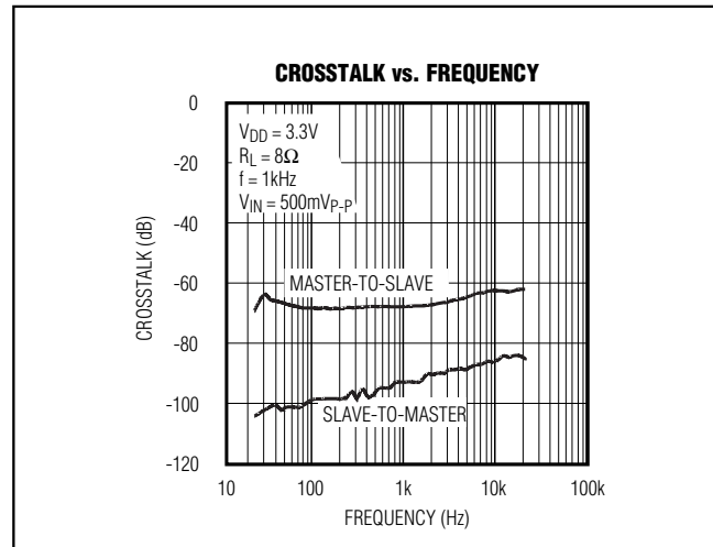
Figure 9. Master-Slave Crosstalk
