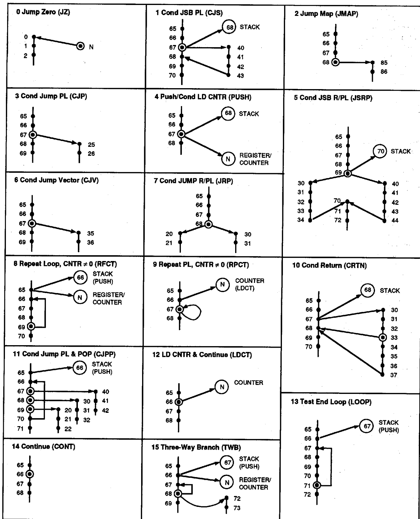
Figure 1. IDT49C410 Flow Diagrams
