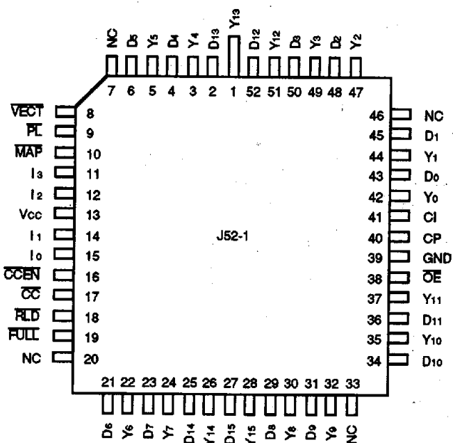
PLCC TOP VIEW
