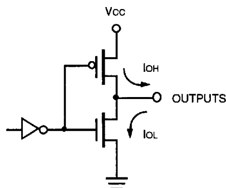
Figure 3. Output Structure
