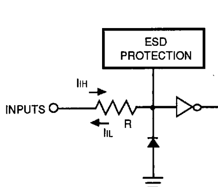
Figure 2. Input Structure
