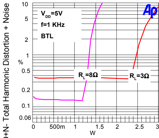
Po - Output Power Figure 4
