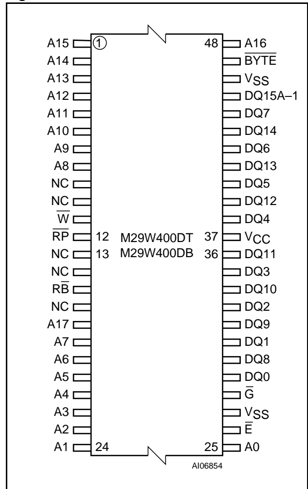
Figure 4. TSOP Connections
