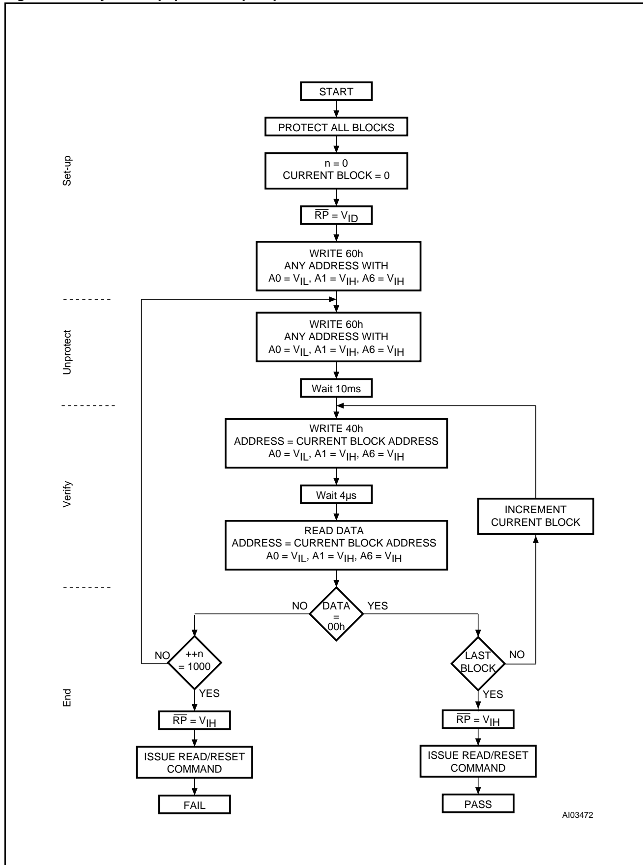
Figure 22. In-System Equipment Chip Unprotect Flowchart
