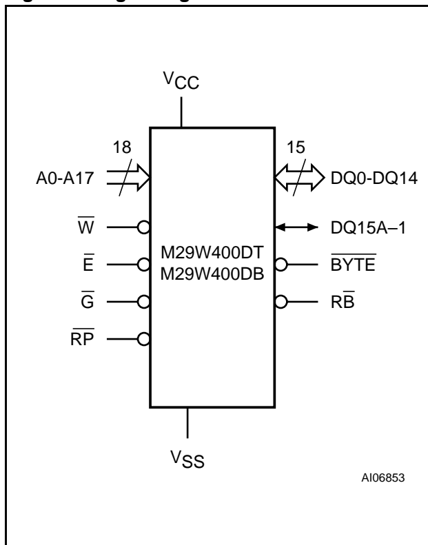
Figure 2. Logic Diagram
