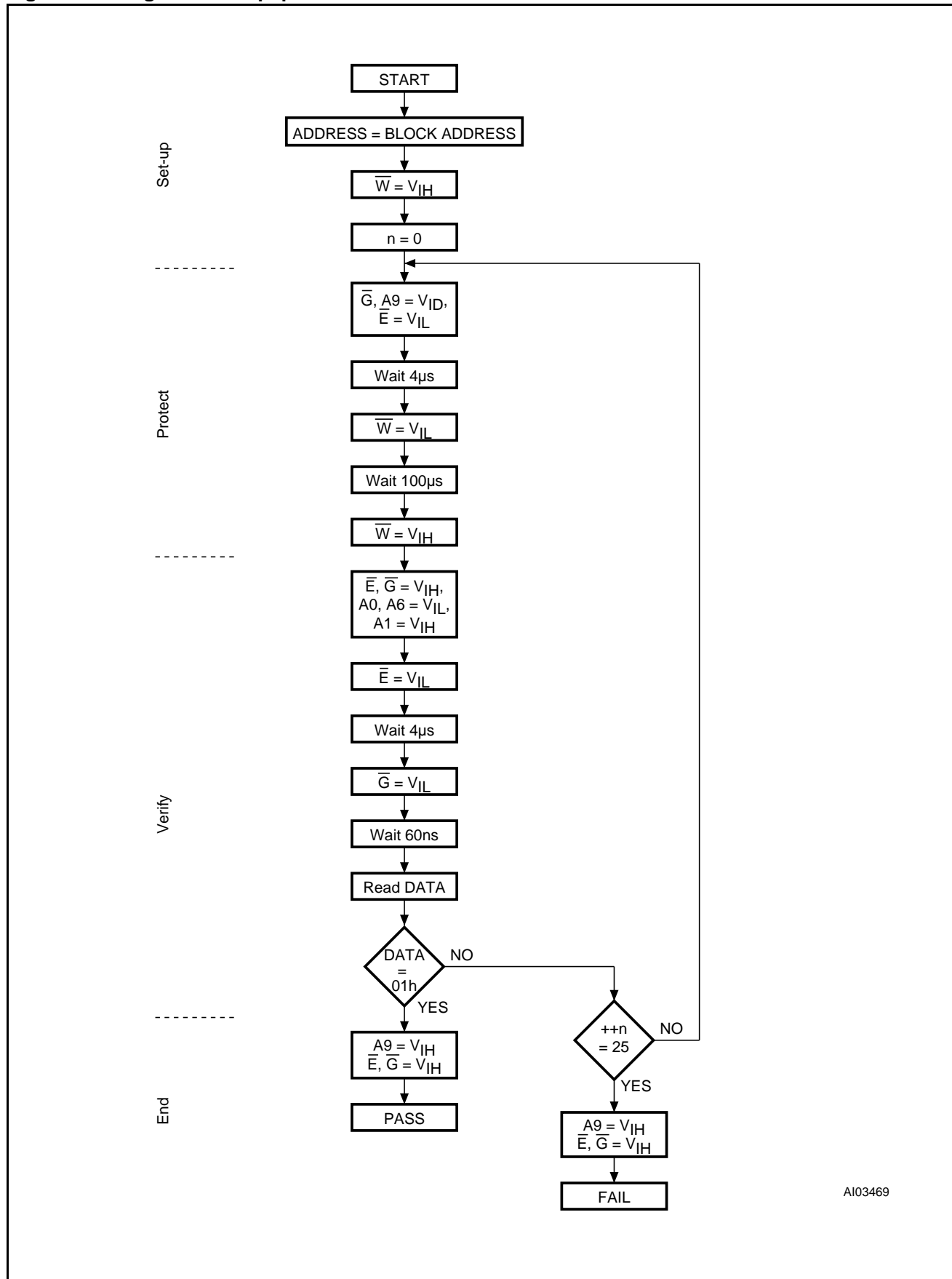
Figure 19. Programmer Equipment Block Protect Flowchart
