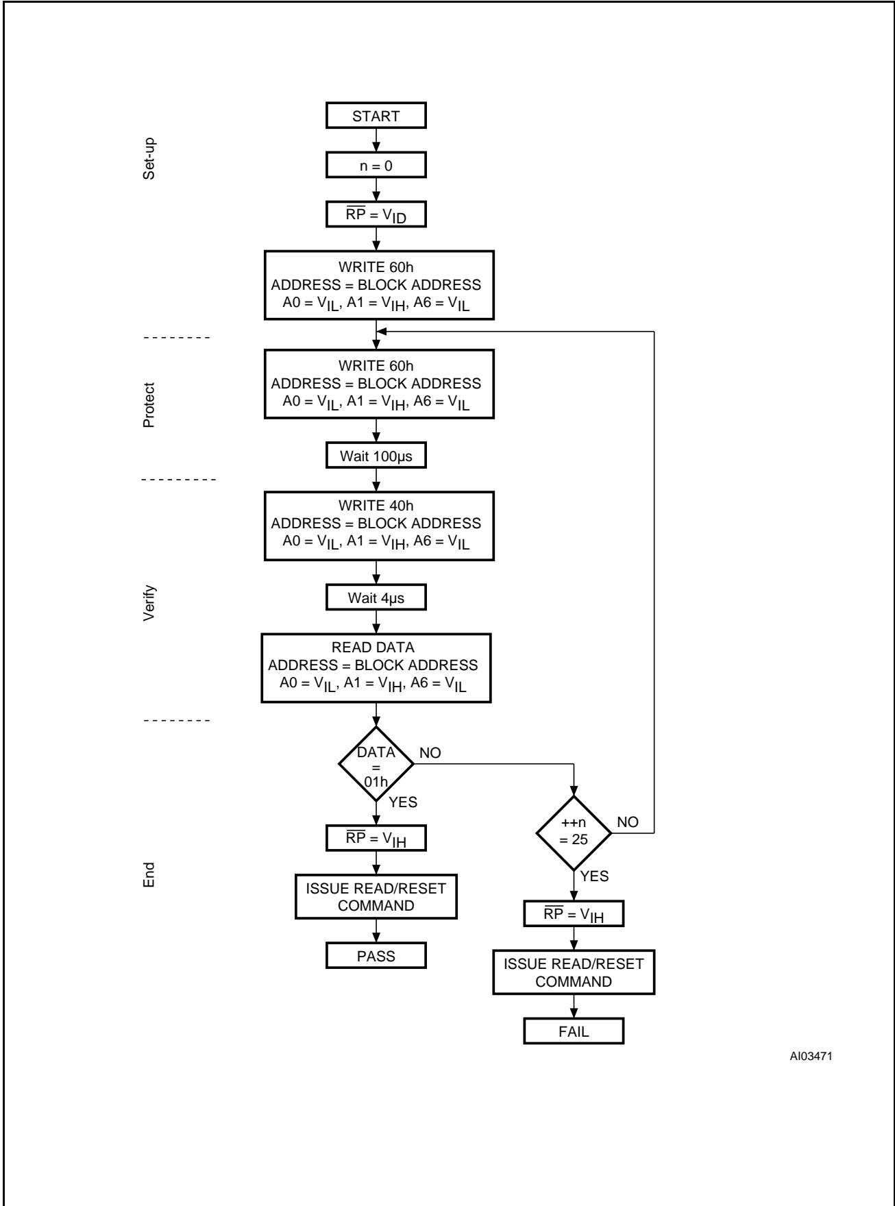
Figure 21. In-System Equipment Block Protect Flowchart
