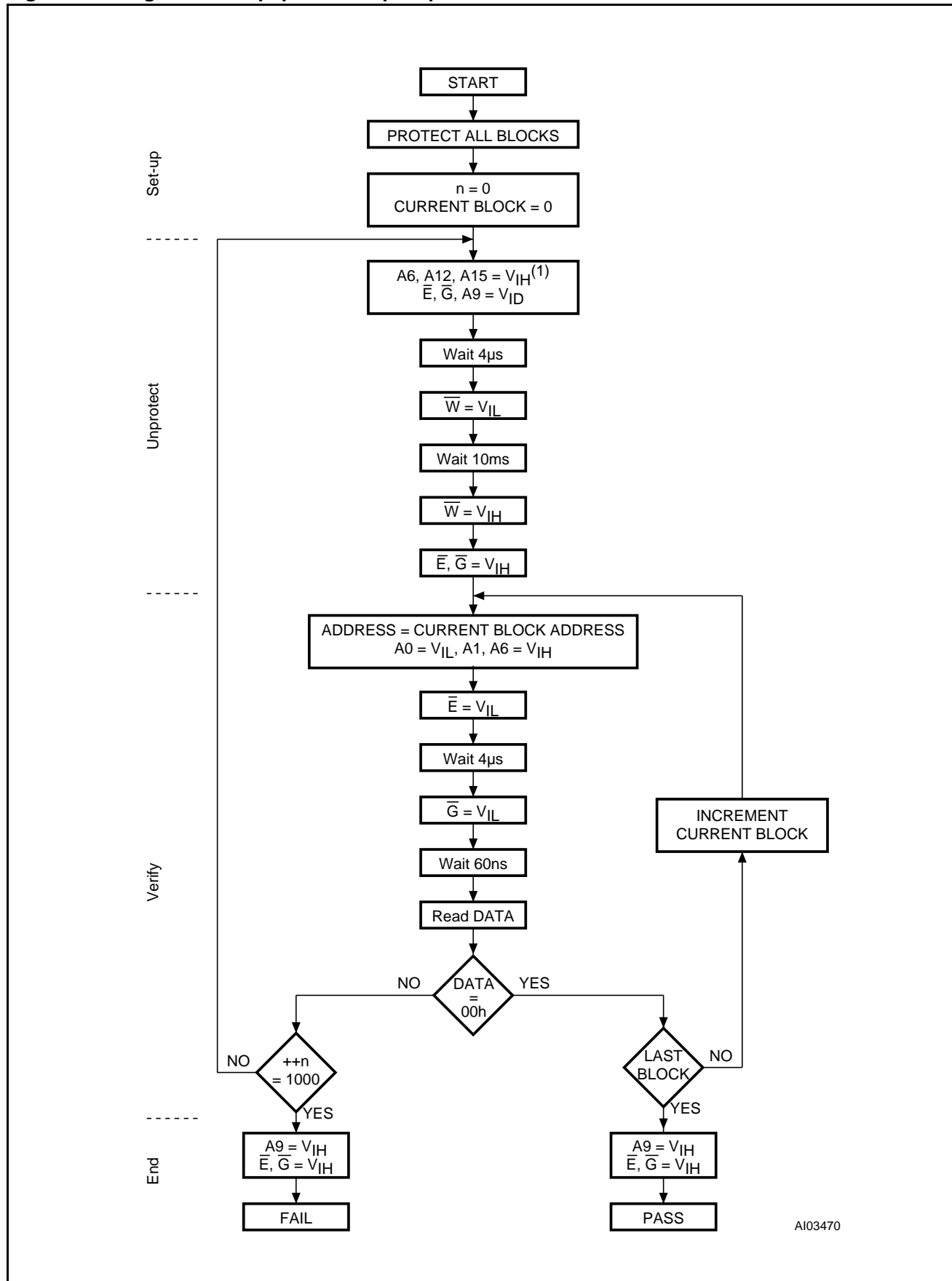
Figure 20. Programmer Equipment Chip Unprotect Flowchart
