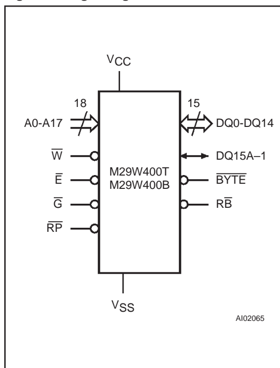
Figure 1. Logic Diagram
