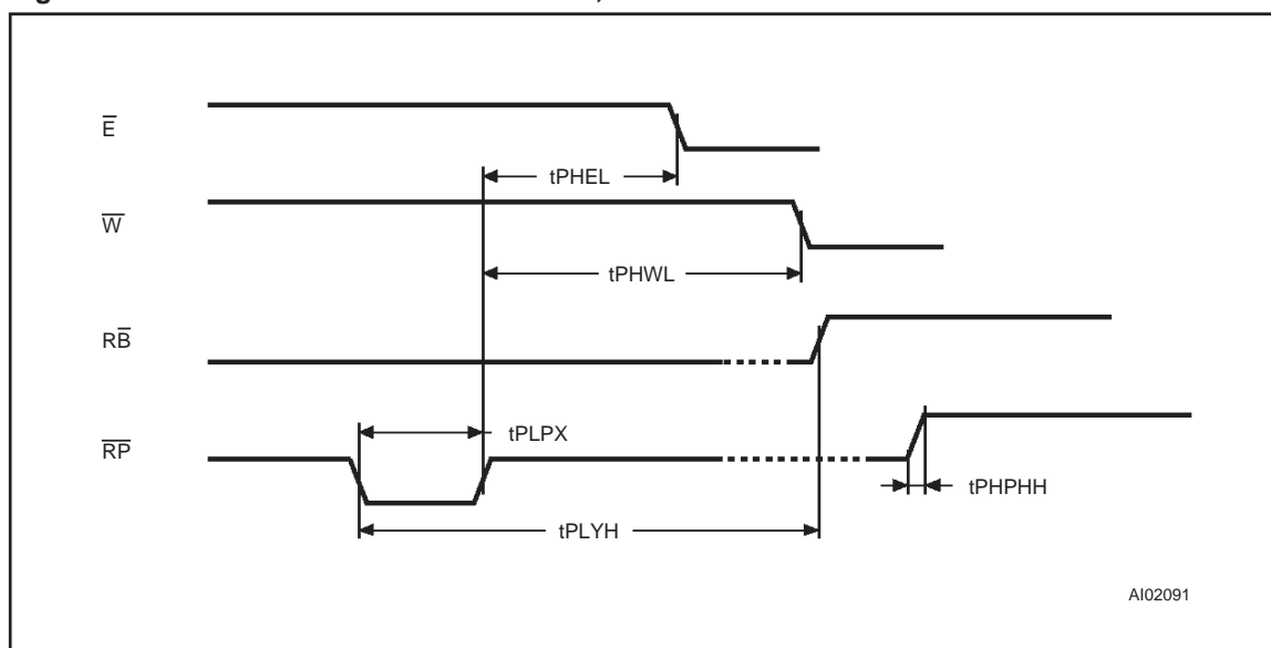
Figure 9. Read and Write AC Characteristics, \overline{RP} Related
