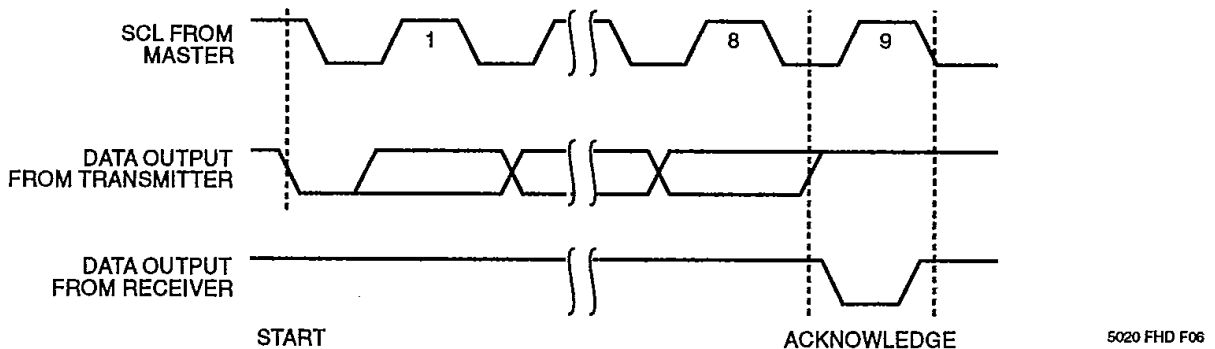
Figure 4. Acknowledge Timing
