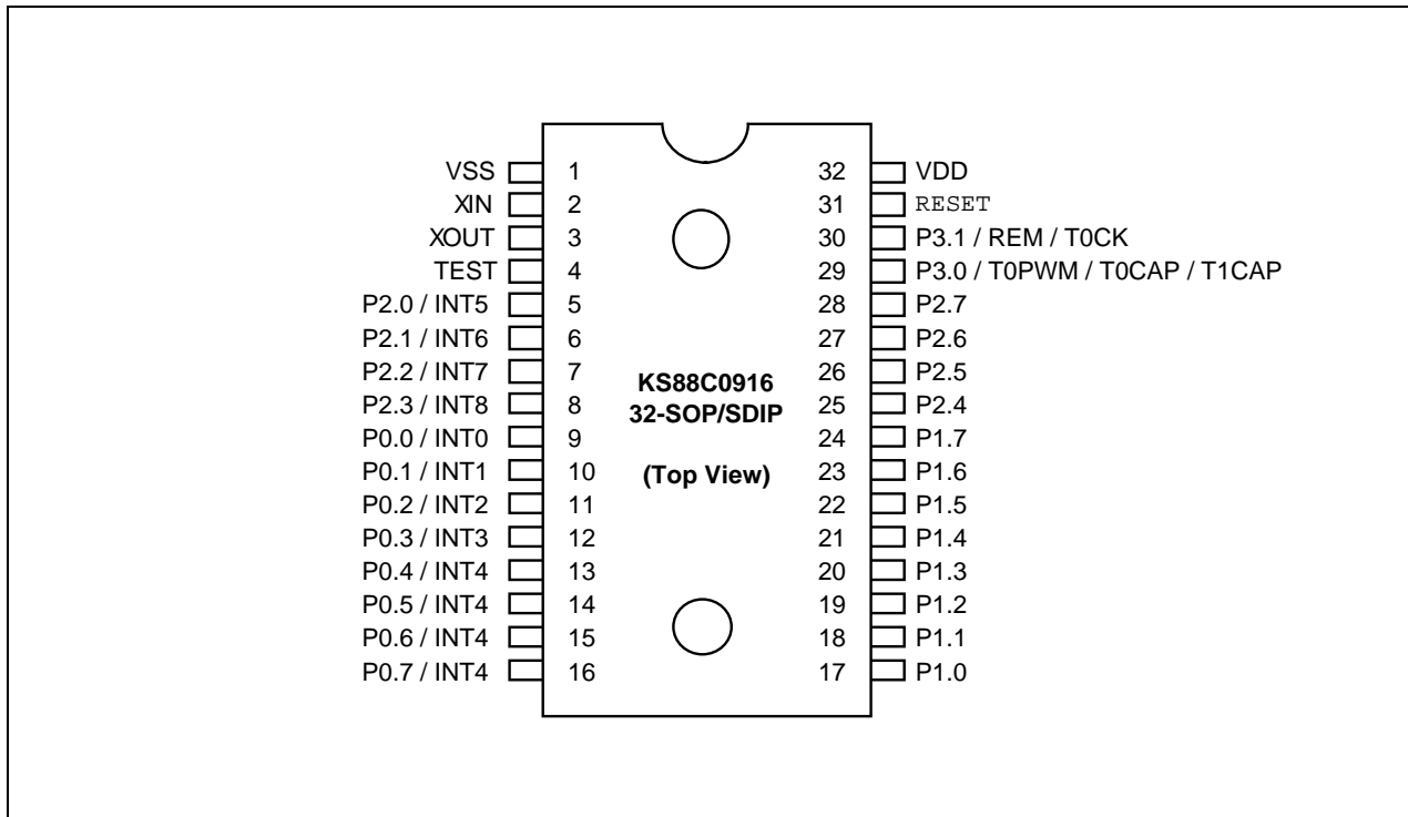
Figure 1-3. Pin Assignment Diagram (32-Pin SOP/SDIP Package)
