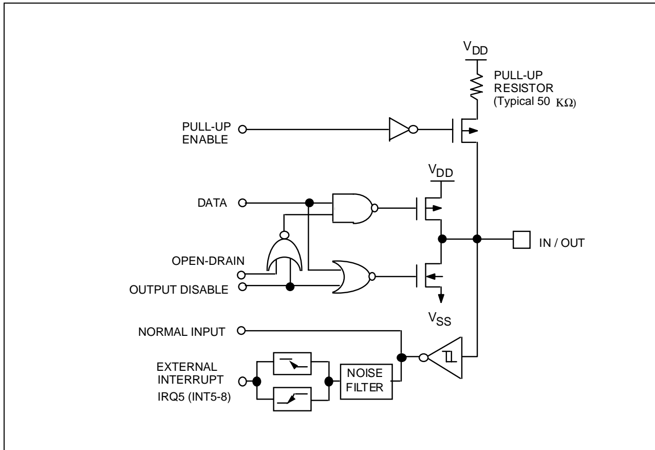
Figure 1-5. Pin Circuit Type 2 (Ports 2.0-2.3)
