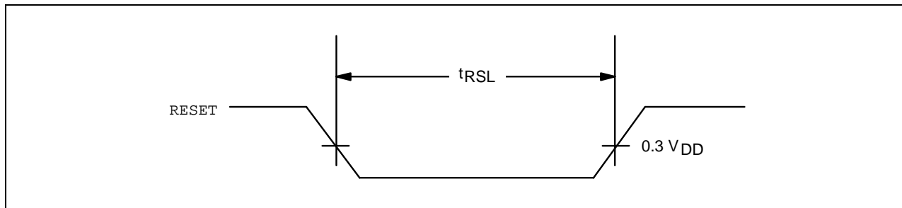
Figure 14-4. Input Timing for RESET
