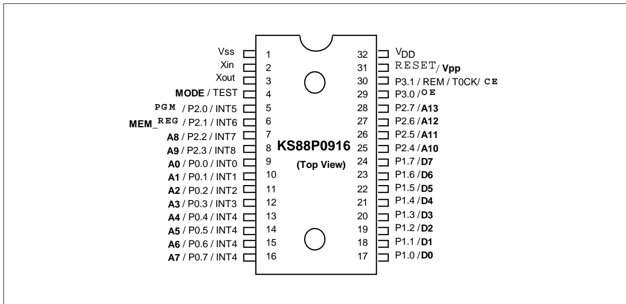
Figure 13–1. KS88P0916 Pin Assignments
