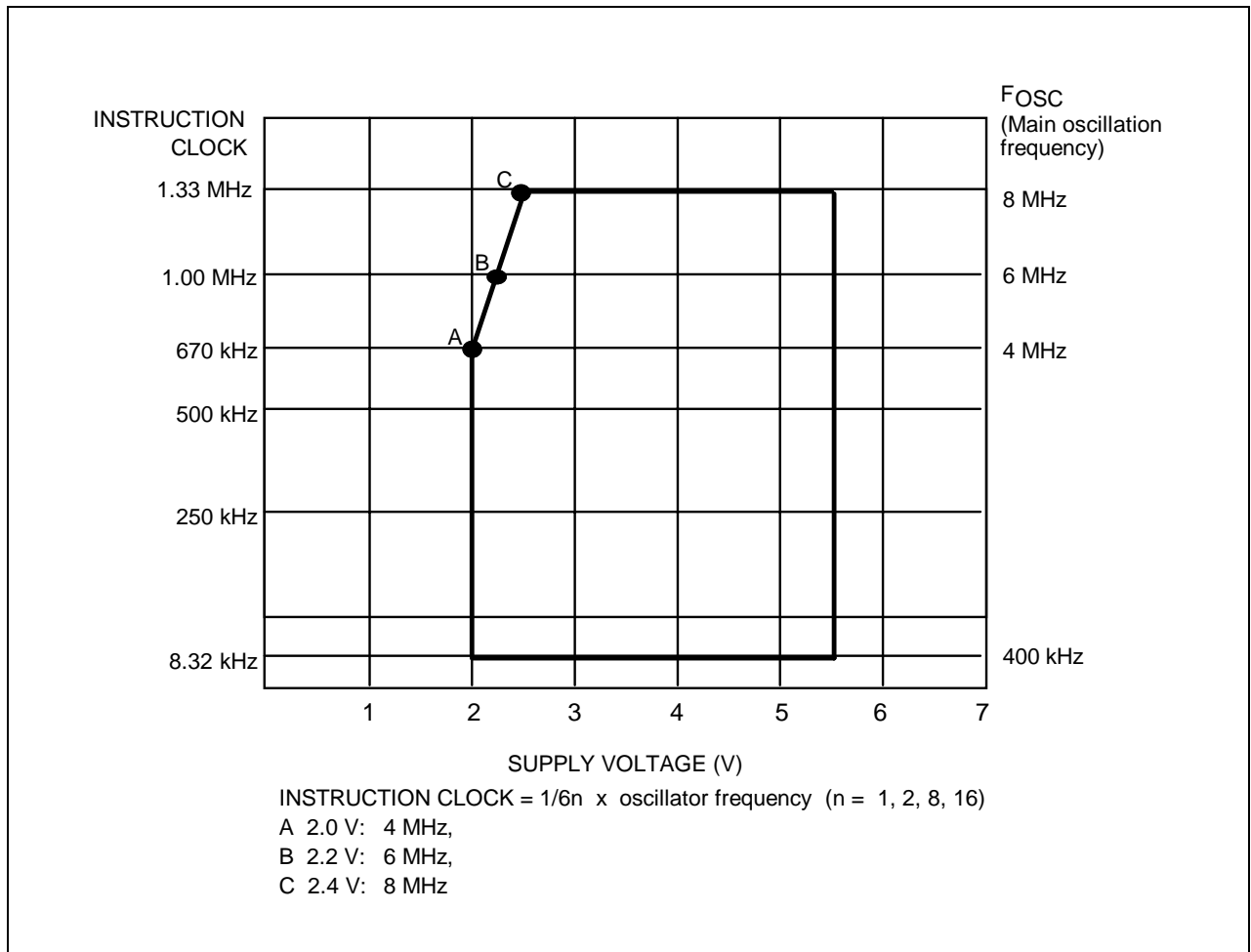
Figure 14-5. Operating Voltage Range
