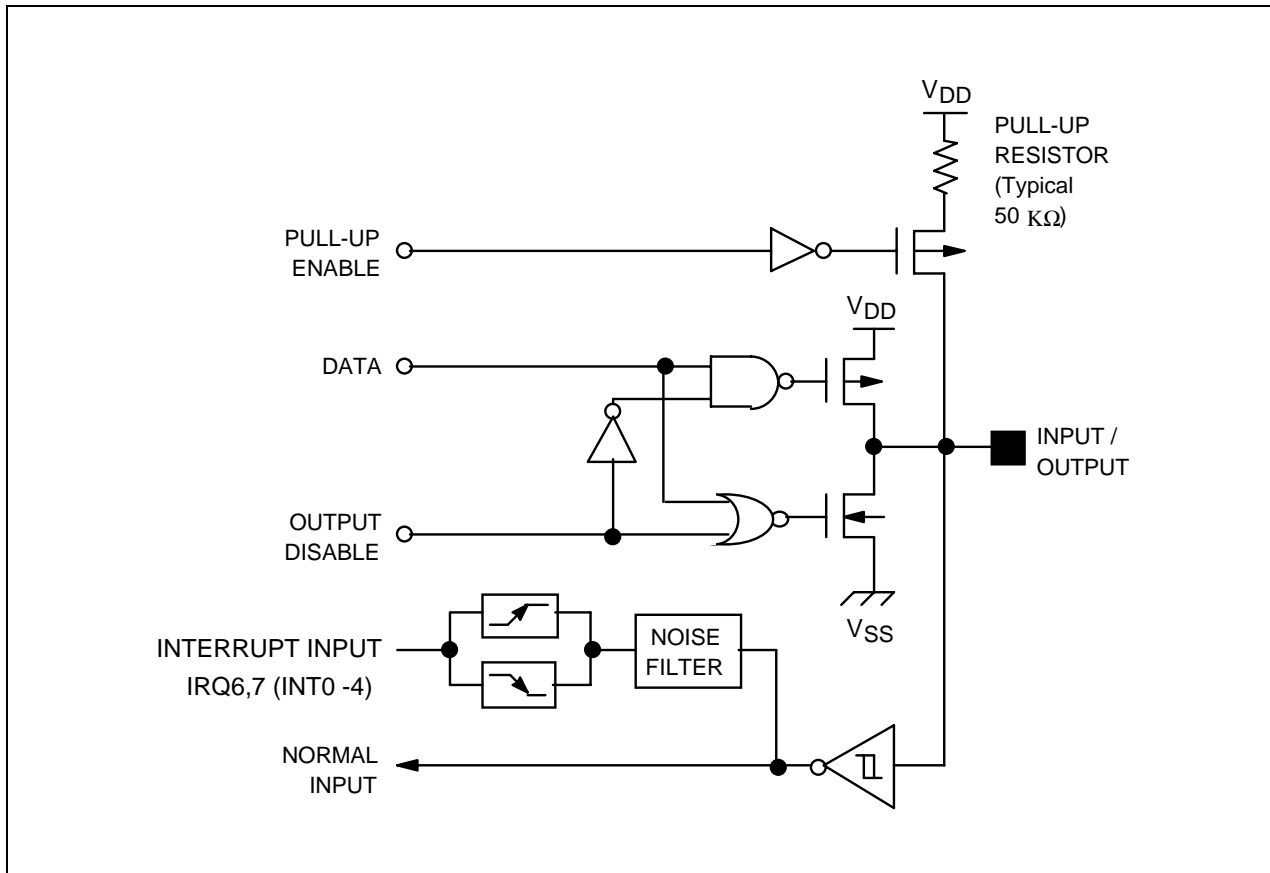
Figure 1-4. Pin Circuit Type 1 (Port 0)
