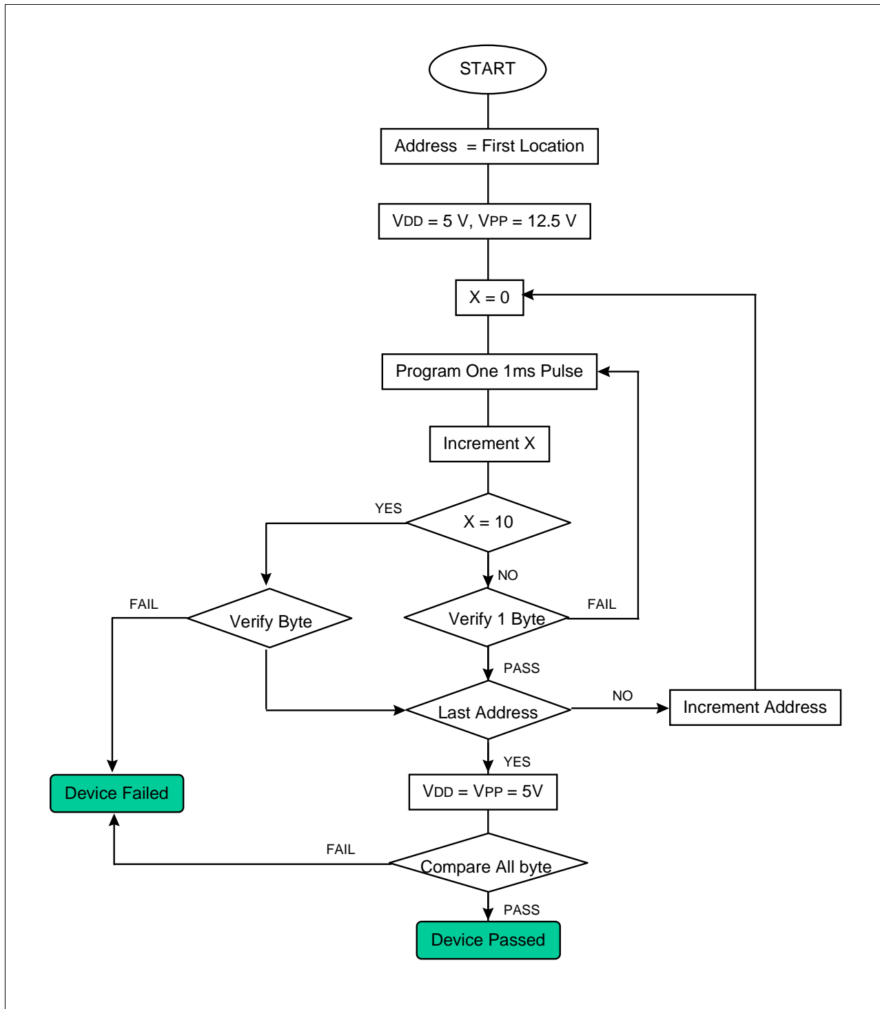
Figure 13-4. OTP Programming Algorithm
