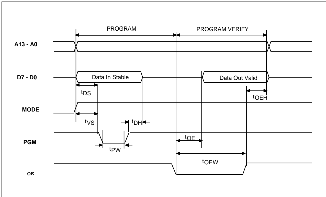
Figure 13-3. Program Memory Write Timing
