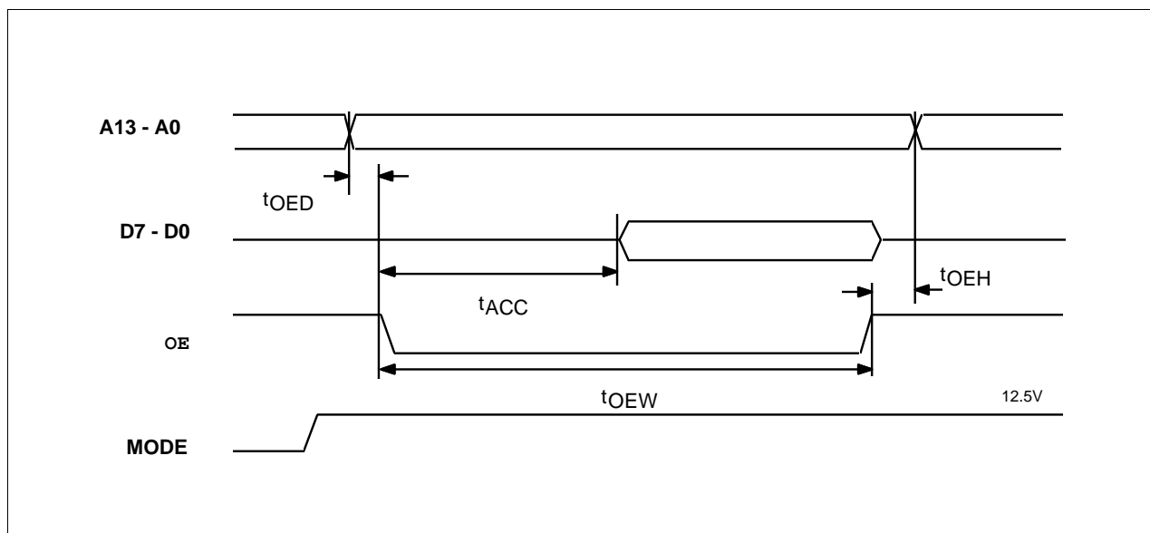
Figure 13-2. OTP Read Timing
