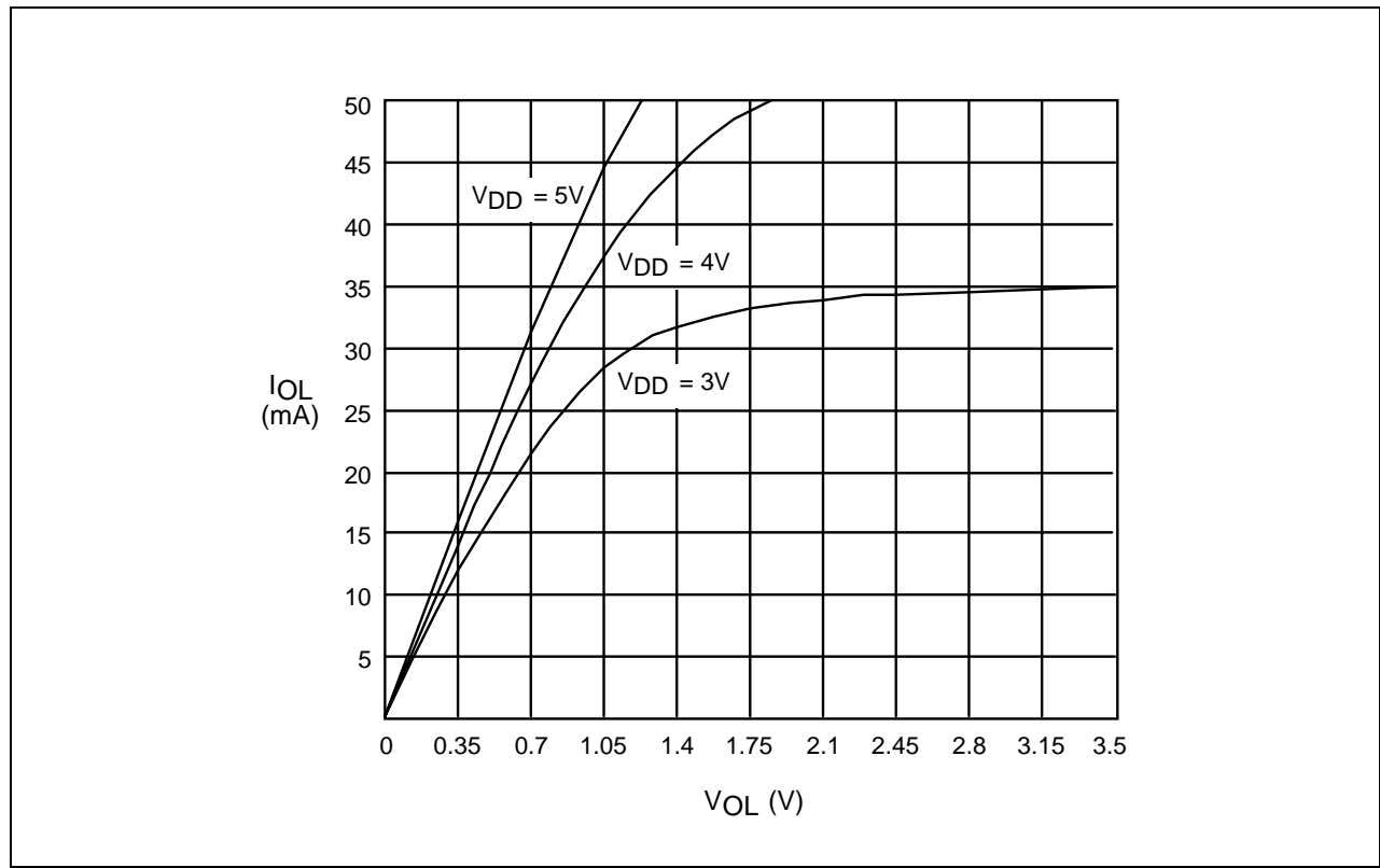
Figure 14-11. I OL vs. V OL (Port 3)
