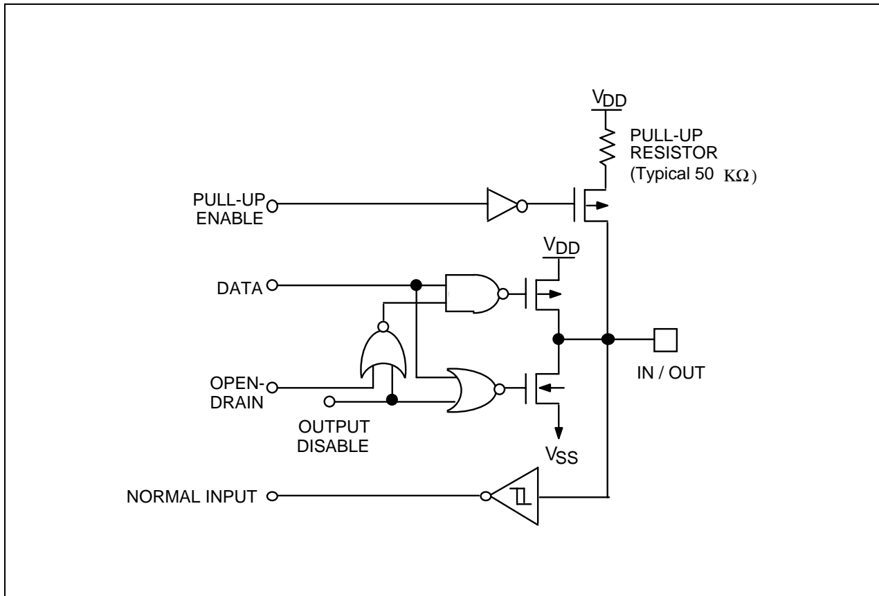
Figure 1-6. Pin Circuit Type 3 (Ports 1 and P2.4–P2.7)
