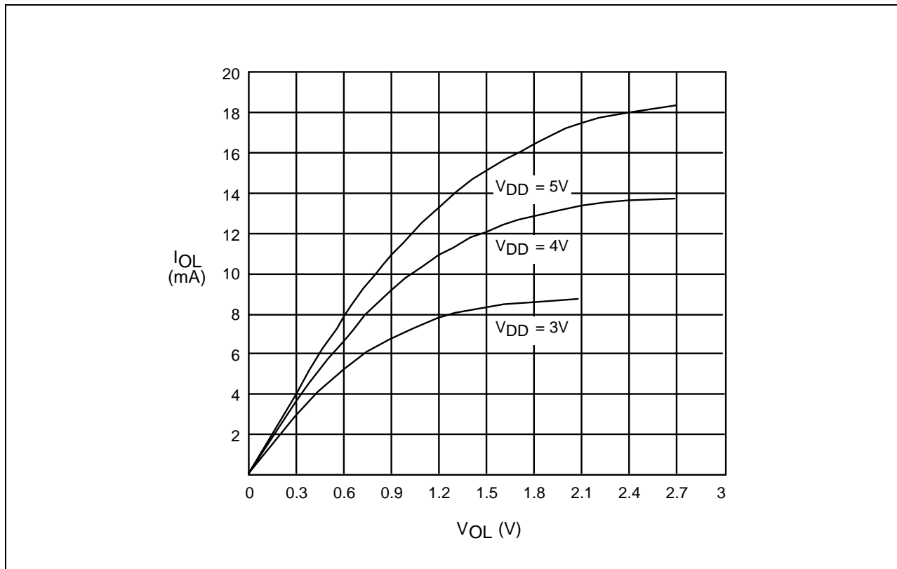
Figure 14-9. I_{OL} vs. V_{OL} (Port 0)
