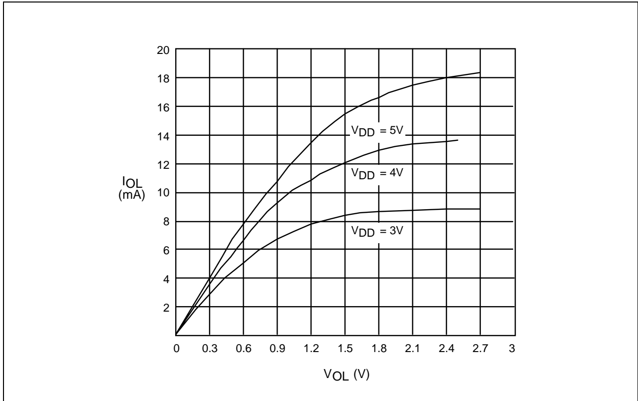
Figure 14-10. I_{OL} vs. V_{OL} (Port 2)
