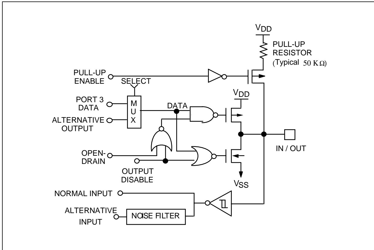
Figure 1-7. Pin Circuit Type 4 (Port 3)
