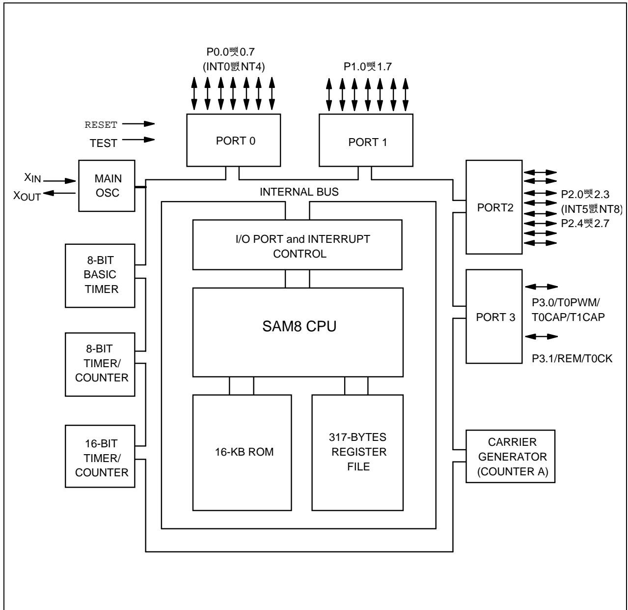
Figure 1-2. Block Diagram
