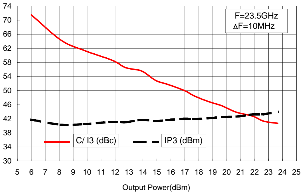
C/I3 & IP3 versus total output power @ 23.5GHz
