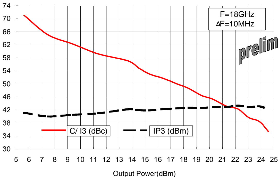
C/I3 & IP3 versus total output power @ 18GHz
