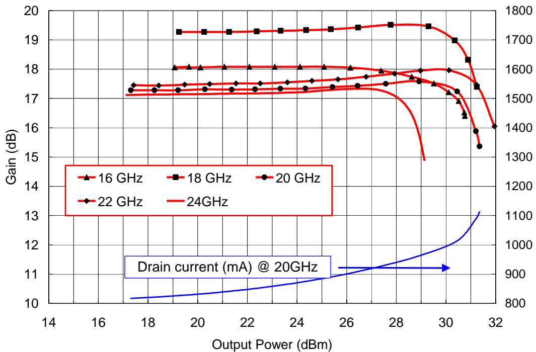
Output power versus frequency & Drain current @ 20GHz
