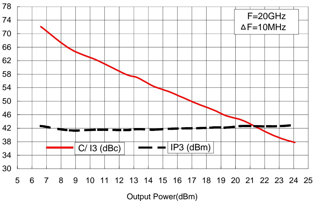
C/I3 & IP3 versus total output power @ 20GHz
