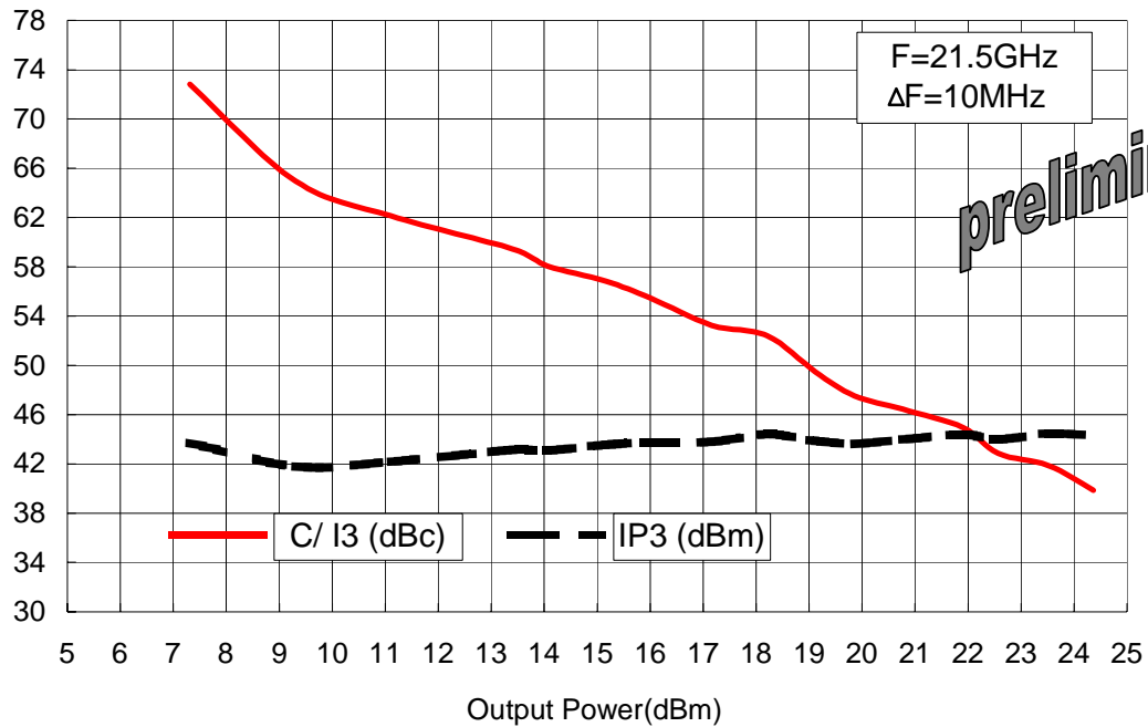
C/I3 & IP3 versus total output power @ 21.5GHz
