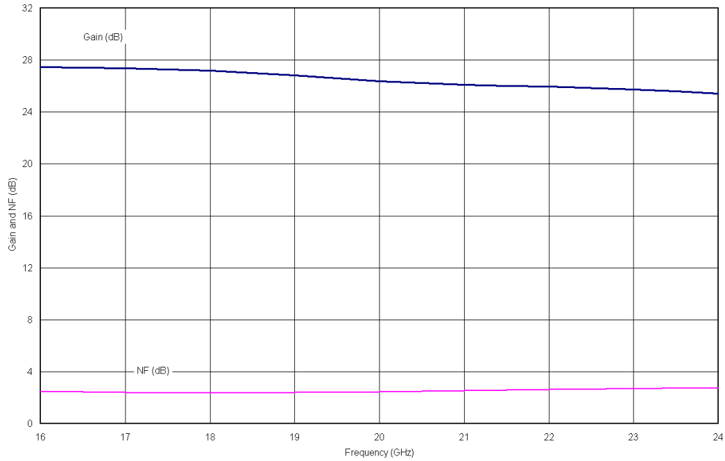
Gain & Noise Figure versus frequency
