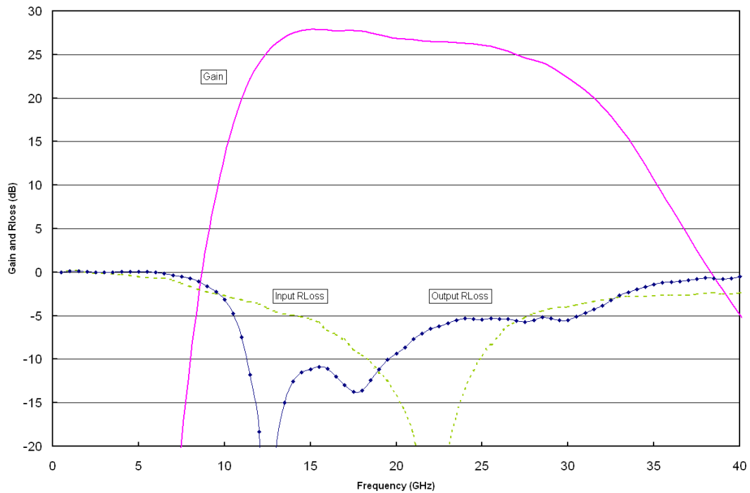
Typical on-wafer Gain & Return Loss
