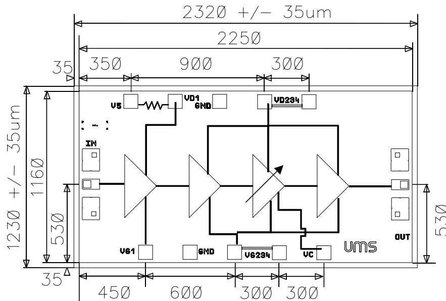
Bonding pad positions ( Chip thickness : 100μm. All dimensions are in micrometers )
