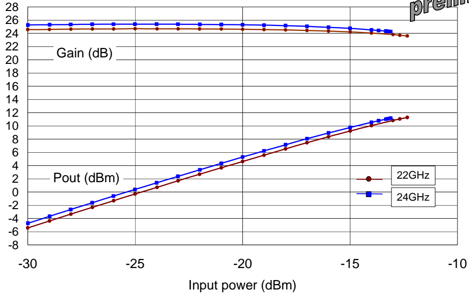
Gain & Output power @ 22-24 GHz
