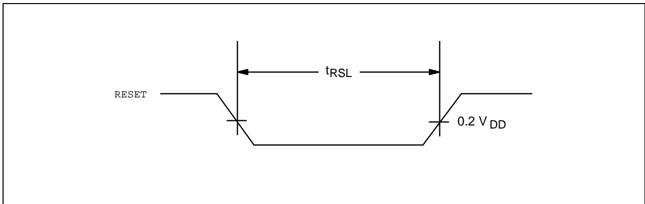
Figure 19-2. Input Timing for RESET
