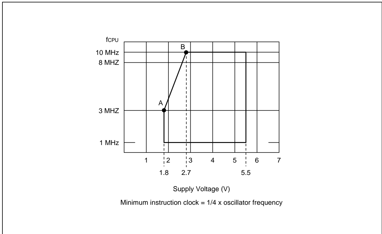
Figure 19-8. Operating Voltage Range
