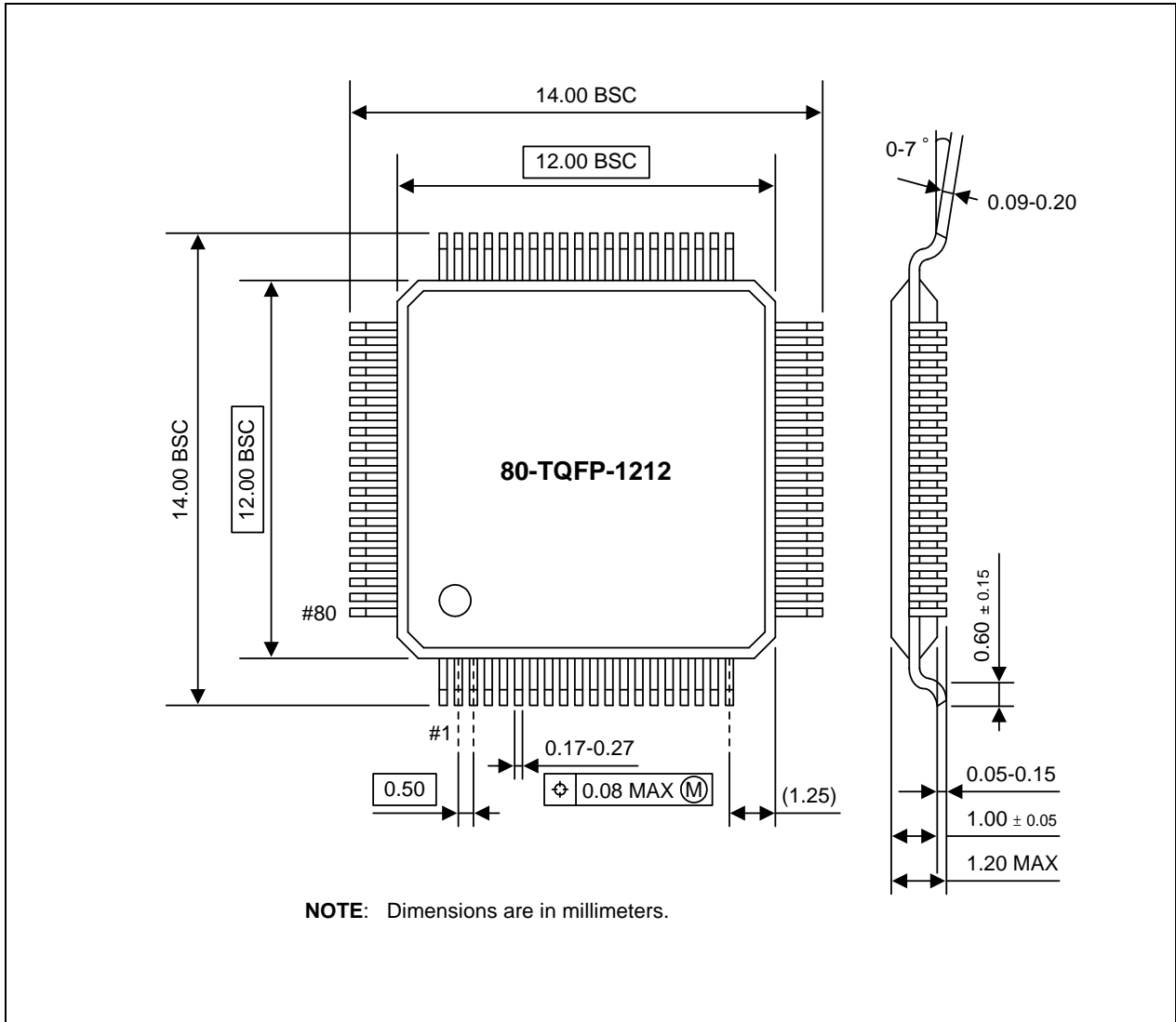
Figure 20-2. 80-Pin TQFP 1212 Package Dimensions
