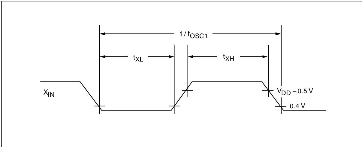
Figure 19-7. Clock Timing Measurement at X IN
