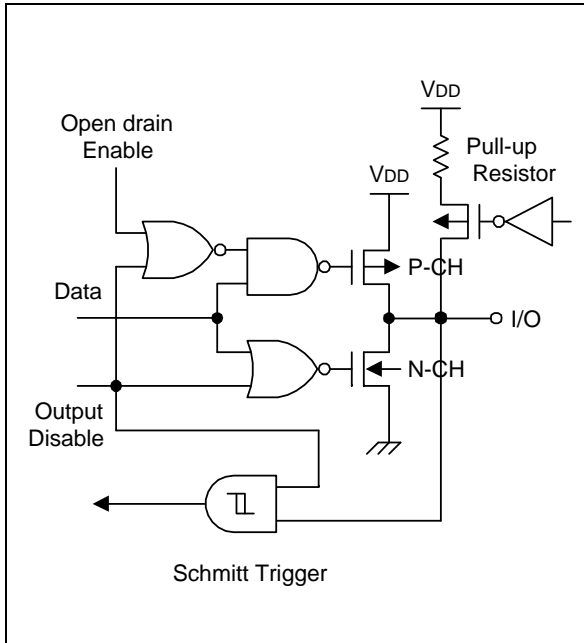
Figure 1-7. Pin Circuit Type E-2 (P1)
