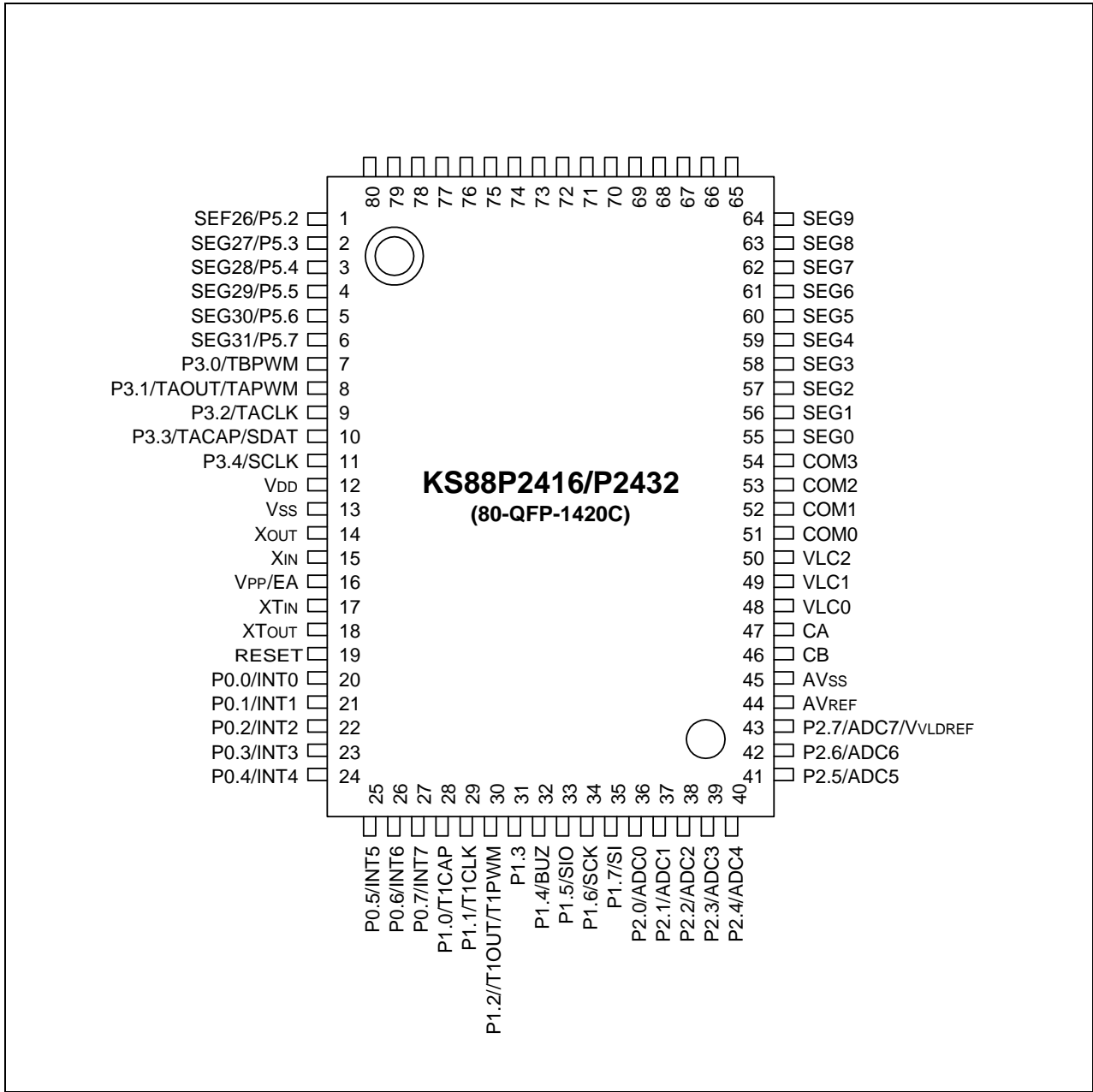
Figure 21-1. KS88P2416/P2432 Pin Assignments (80-QFP Package)
