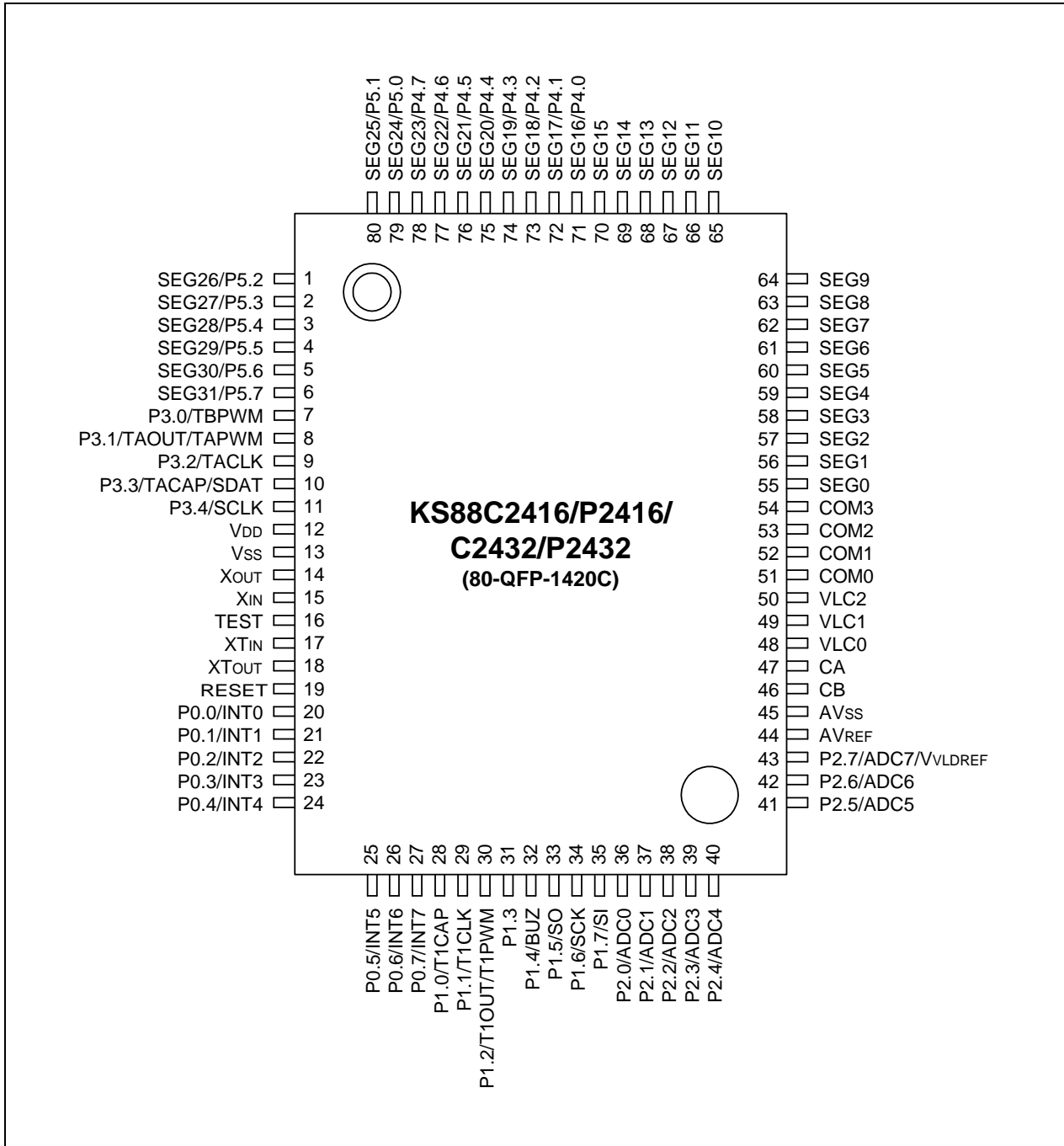
Figure 1-2. KS88C2416/2432 Pin Assignment (80-QFP)
