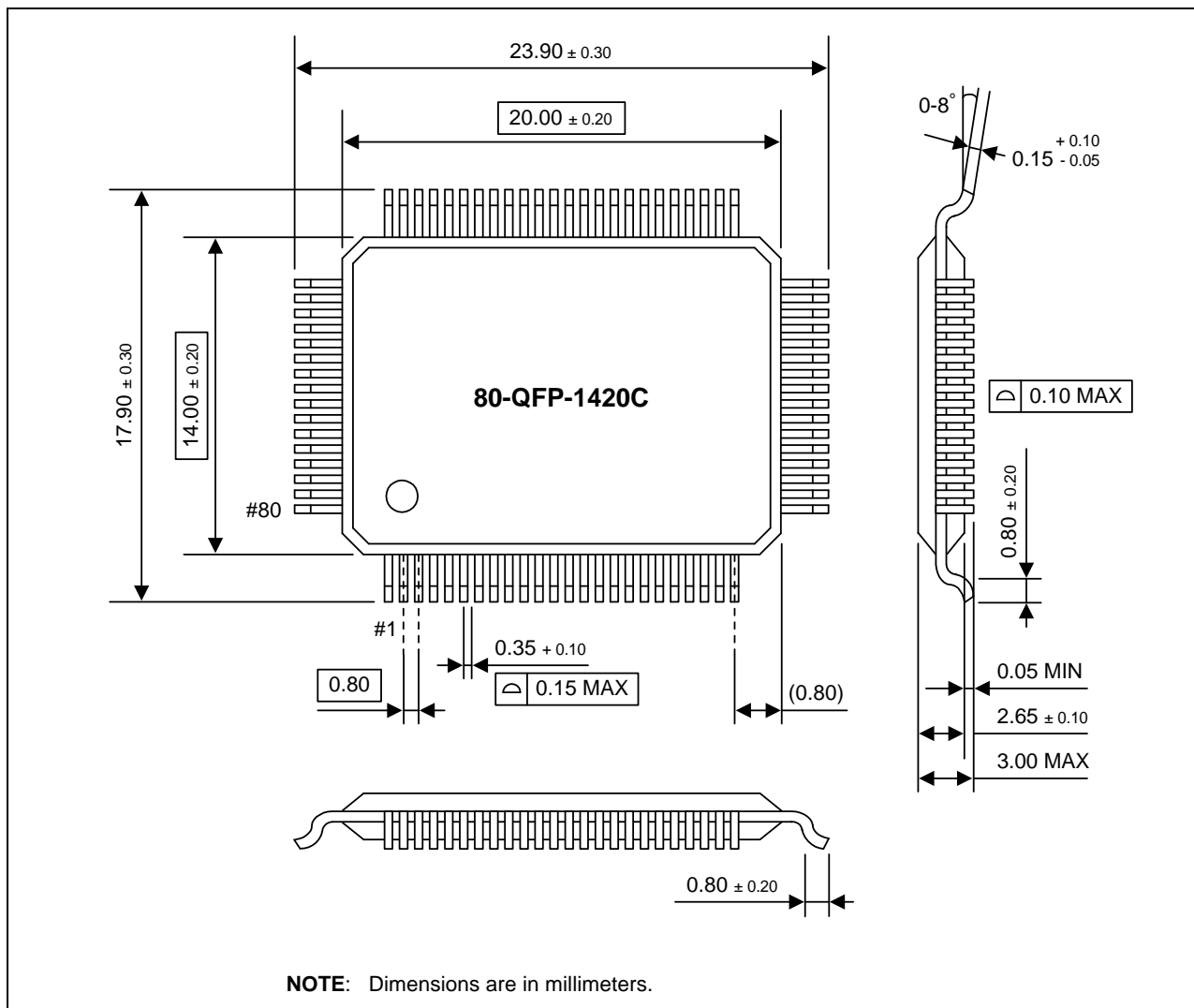
Figure 20-1. 80-Pin QFP 1420C Package Dimensions
