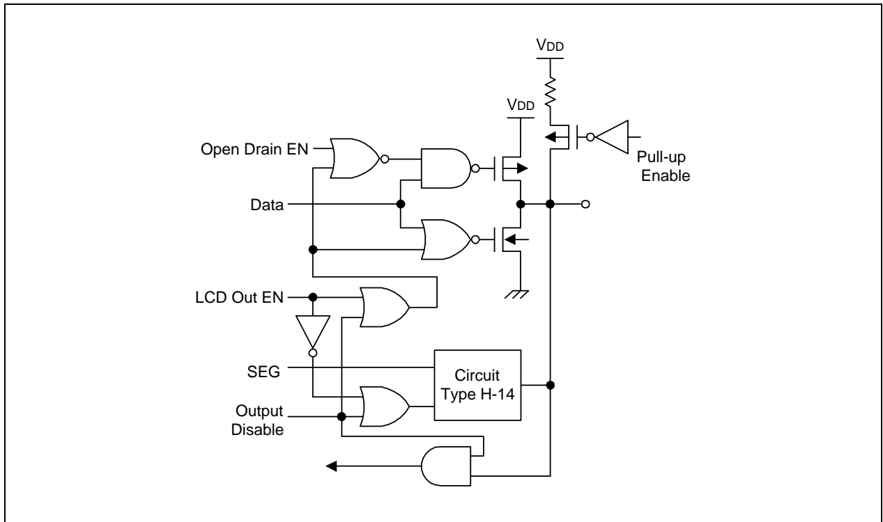
Figure 1-12. Pin Circuit Type H-14 (P4, P5)
