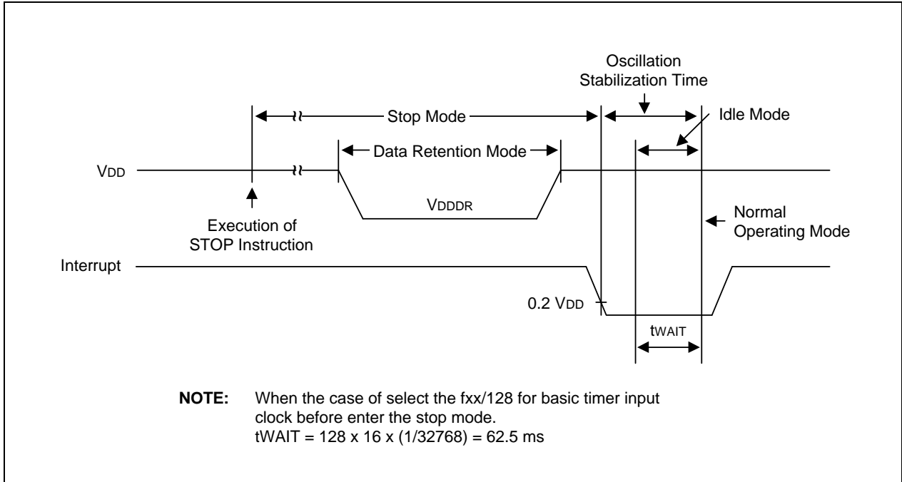
Figure 19-5. Stop Mode(sub) Release Timing Initiated by Interrupts
