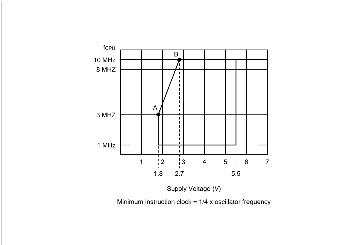
Figure 21-2. Operating Voltage Range
