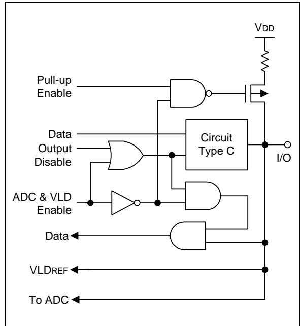
Figure 1-9. Pin Circuit Type F-18 (P2.7/VLD REF )
