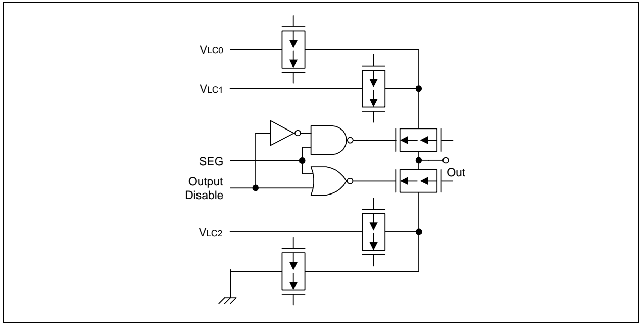
Figure 1-11. Pin Circuit Type H-4
