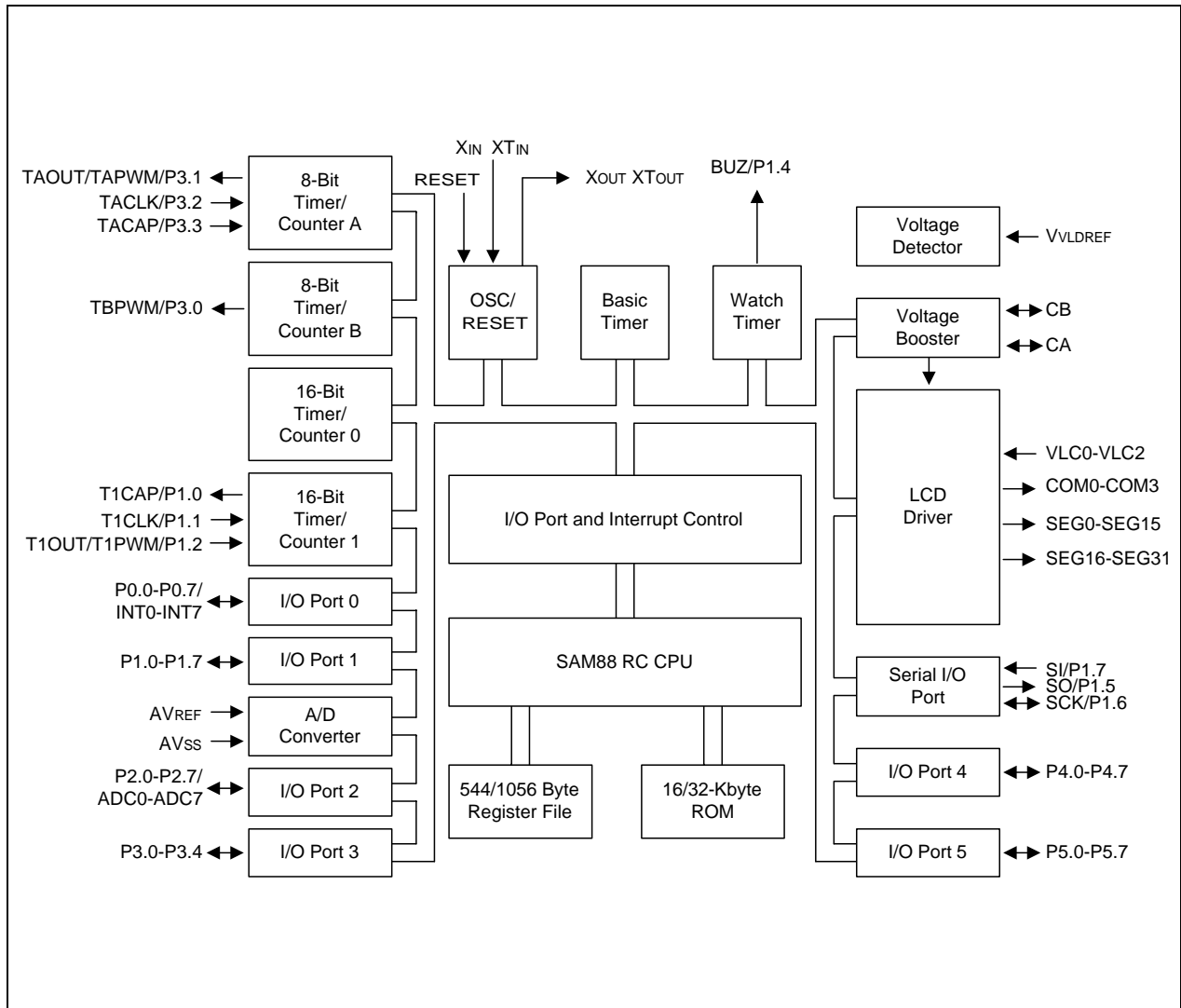
Figure 1-1. KS88C2416/2432 Block Diagram
