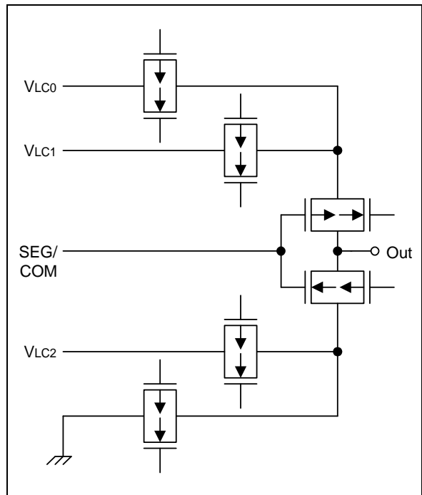
Figure 1-10. Pin Circuit Type H (SEG/COM)
