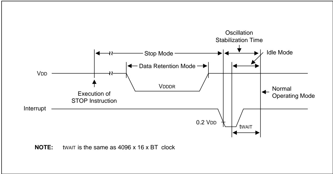
Figure 19-4. Stop Mode(main) Release Timing Initiated by Interrupts
