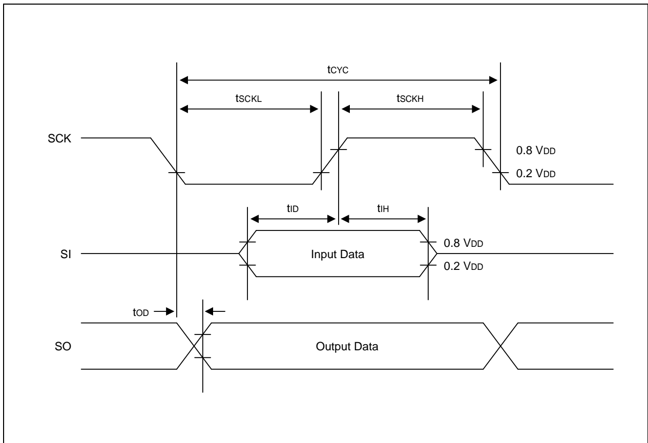
Figure 19-6. Serial Data Transfer Timing
