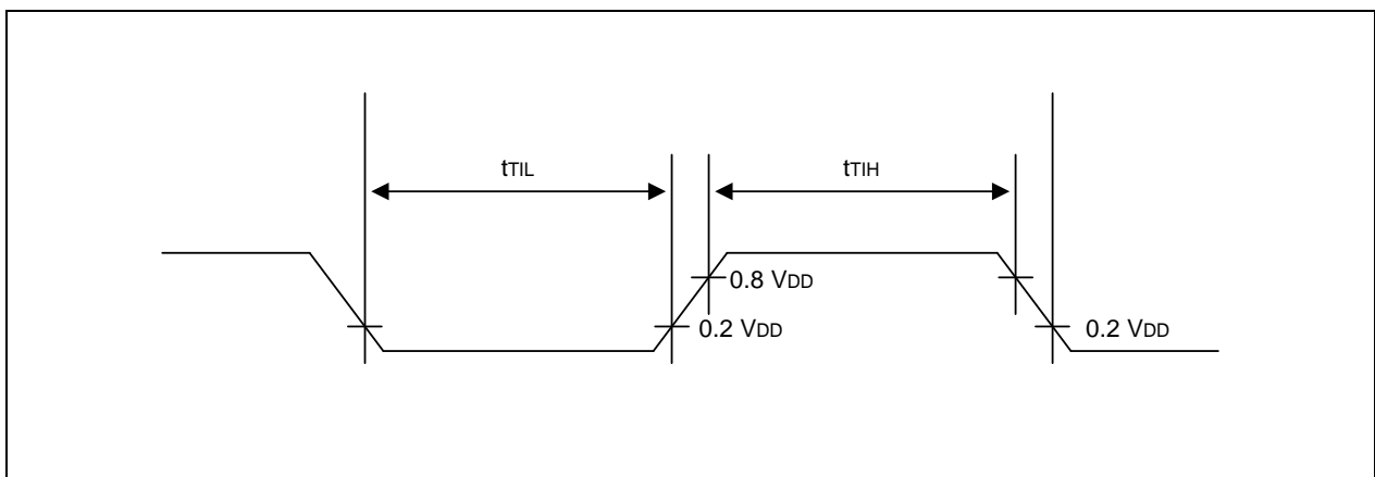
Figure 19-1. Input Timing for External Interrupts (Ports 0)
