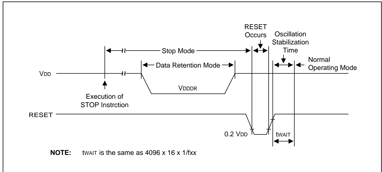
Figure 19-3. Stop Mode Release Timing Initiated by RESET
