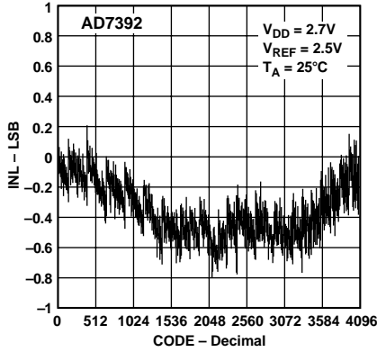
Figure 5. AD7392 Integral Nonlinear Error vs. Code
