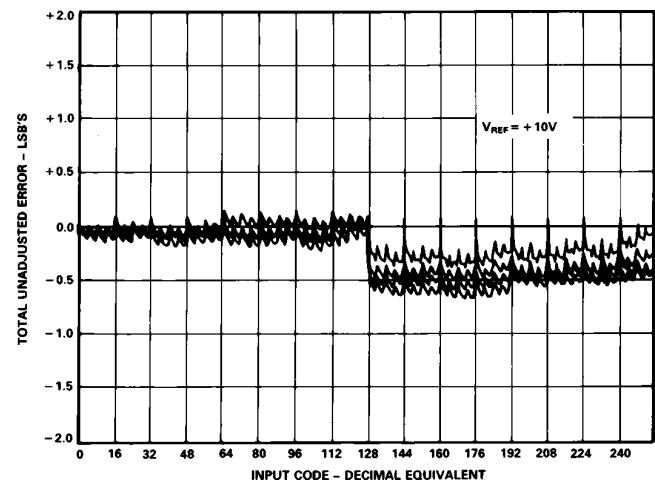
Figure 6. Channel-to-Channel Matching
