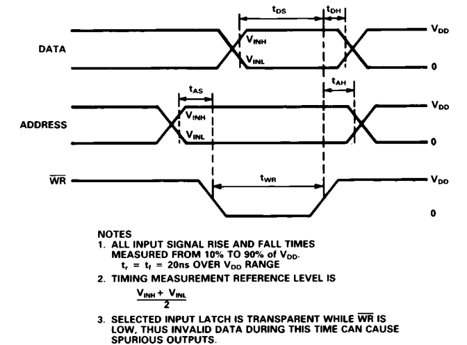
Figure 5. Write Cycle Timing Diagram
