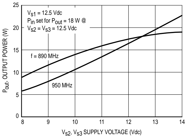
Figure 10. P_{out} versus Supply Voltage
