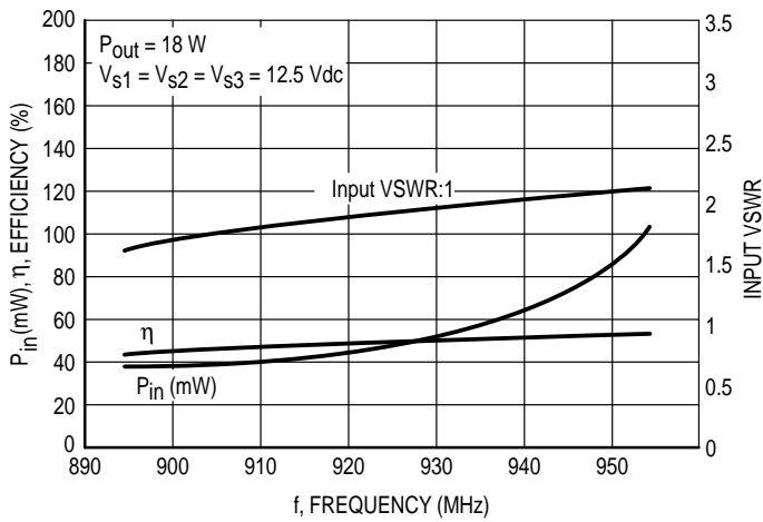
Figure 8. P_{in} VSWR, and Efficiency versus Frequency
