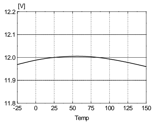
Figure 14. Burst Mode High Voltage vs. Temp
