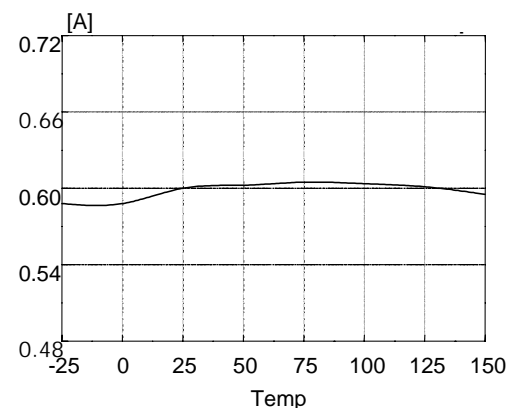
Figure 16. Burst Mode Peak Current vs. Temp
