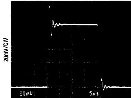
A_V = +1, C_{LOAD} = 1000pF, 5\mu s/DIV
