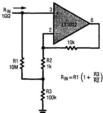
Resistor Multiplier
