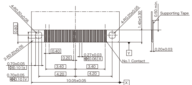
Recommended FPC Dimensions
