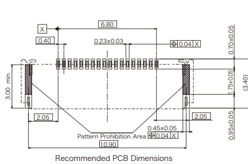
Recommended PCB Dimensions
