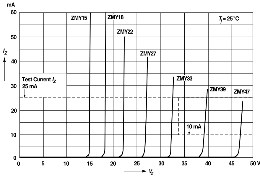
Figure 7. Breakdown Characteristics
