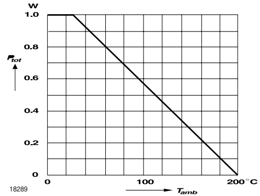
Figure 4. Admissible Power Dissipation vs. Ambient Temperature
