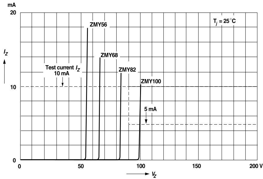
Figure 8. Breakdown Characteristics
