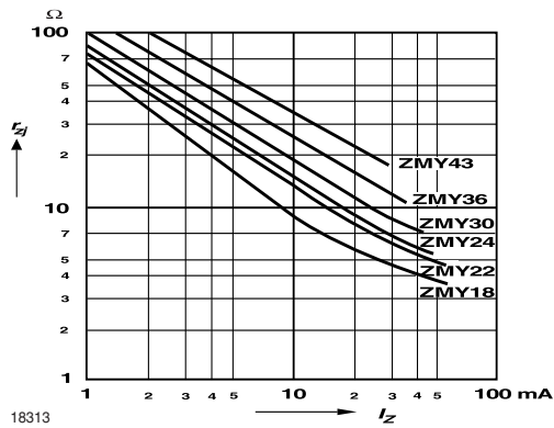
Figure 2. Dynamic Resistance vs. Zener Current
