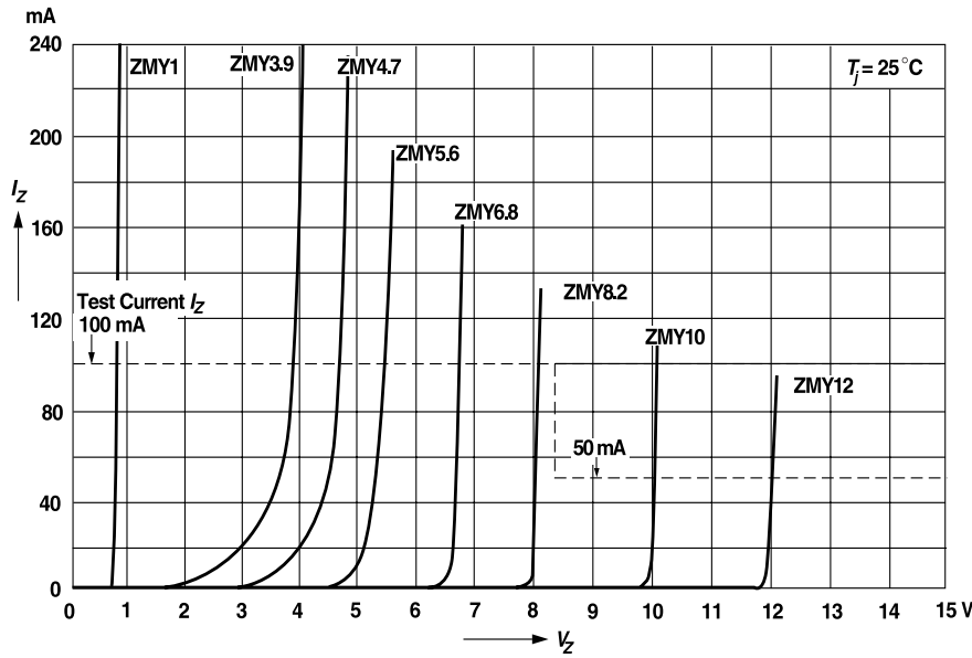
Figure 6. Breakdown Characteristics
