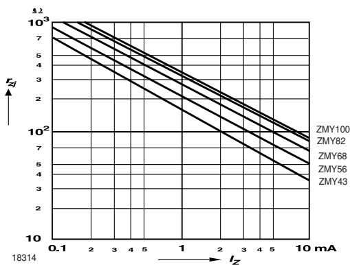
Figure 3. Dynamic Resistance vs. Zener Current
