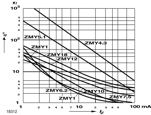
Figure 1. Dynamic Resistance vs. Zener Current
