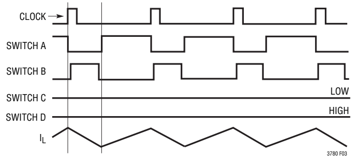
Figure 3. Buck Region ( V_{IN} \gg V_{OUT} )
