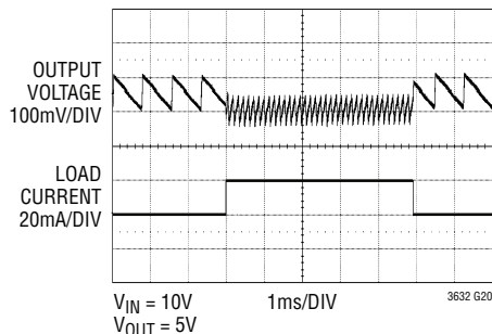
Load Step Transient Response
