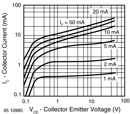
95 10985 Fig. 11 - Collector Current vs. Collector Emitter Voltage
