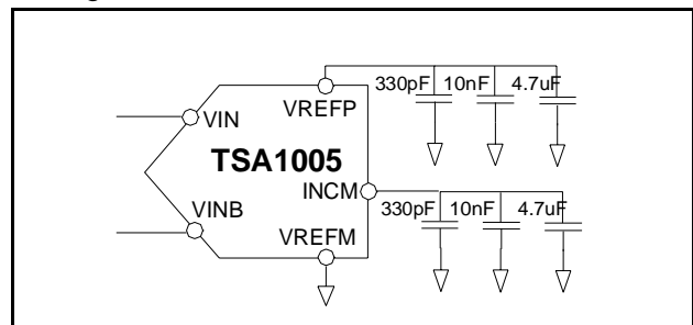
Figure 1: Internal reference and common mode setting
