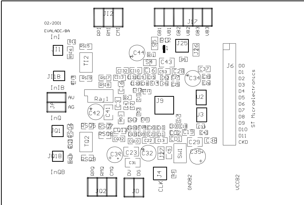
Figure 10: Printed circuit of evaluation board.
