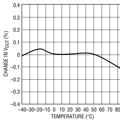
VOUT Variation vs Temperature (Normalized to 25°C)
