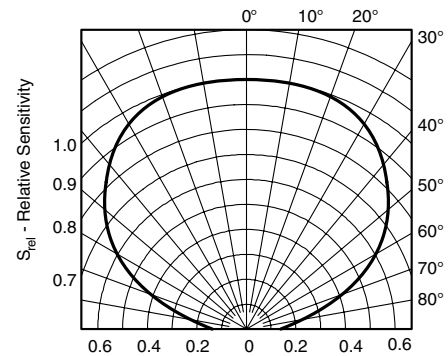
Figure 7. Relative Radiant Sensitivity vs. Angular Displacement
