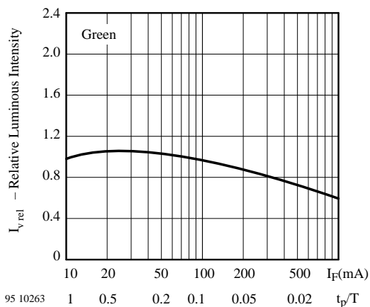
Figure 21. Rel. Lumin. Intensity vs. Forw. Current/Duty Cycle
