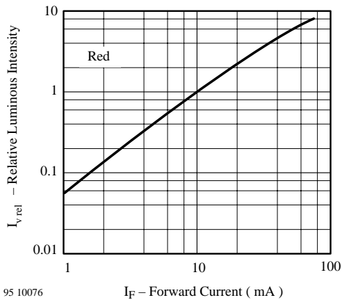
95 10076 Figure 7. Relative Luminous Intensity vs. Forward Current
