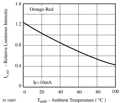
95 10087 Figure 10. Rel. Luminous Intensity vs. Ambient Temperature
