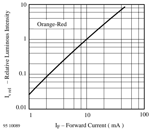
95 10089 Figure 12. Relative Luminous Intensity vs. Forward Current
