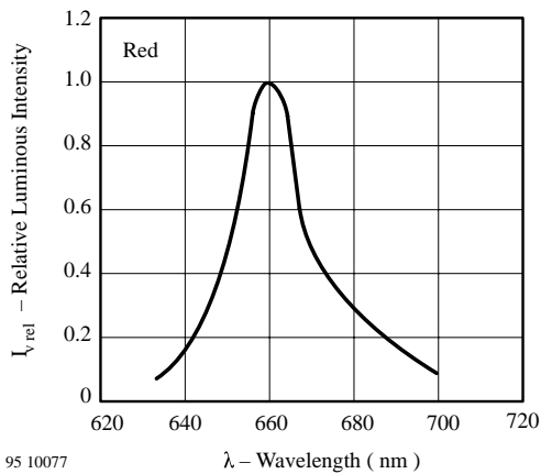
95 10077 Figure 8. Relative Luminous Intensity vs. Wavelength
