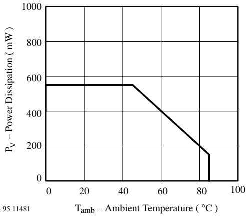
95 11481 Figure 1. Power Dissipation vs. Ambient Temperature
