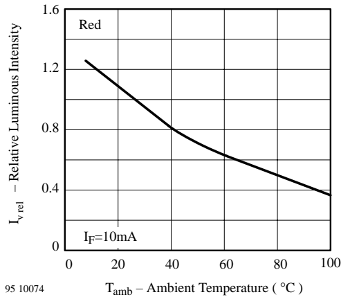
95 10074 Figure 5. Rel. Luminous Intensity vs. Ambient Temperature
