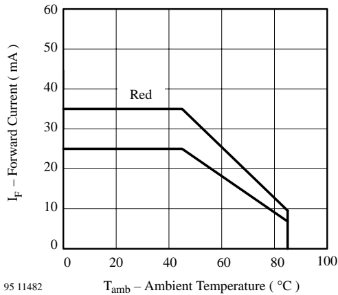
95 11482 Figure 2. Forward Current vs. Ambient Temperature
