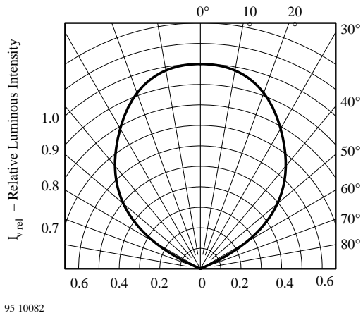
95 10082 Figure 3. Rel. Luminous Intensity vs. Angular Displacement
