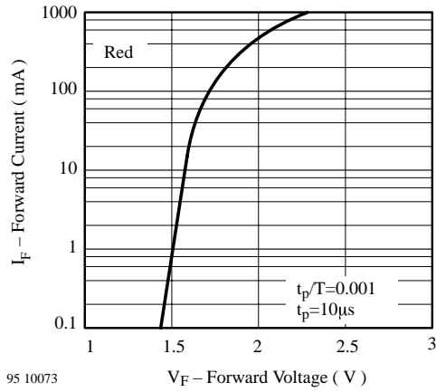
95 10073 Figure 4. Forward Current vs. Forward Voltage
