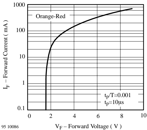
95 10086 Figure 9. Forward Current vs. Forward Voltage
