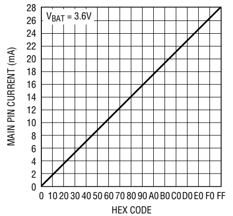
MAIN Pin Current vs Input Code
