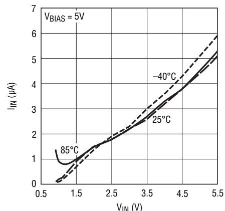
I_{IN} Shutdown Current
