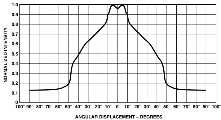
Figure 10. HLMP-P106/-P156.
