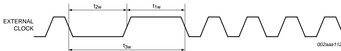
Fig 9. External clock timing.
