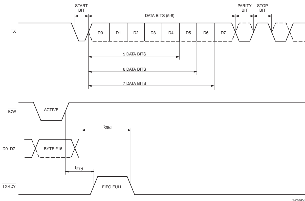
Fig 15. Transmit ready timing in FIFO mode (DMA mode '1').
