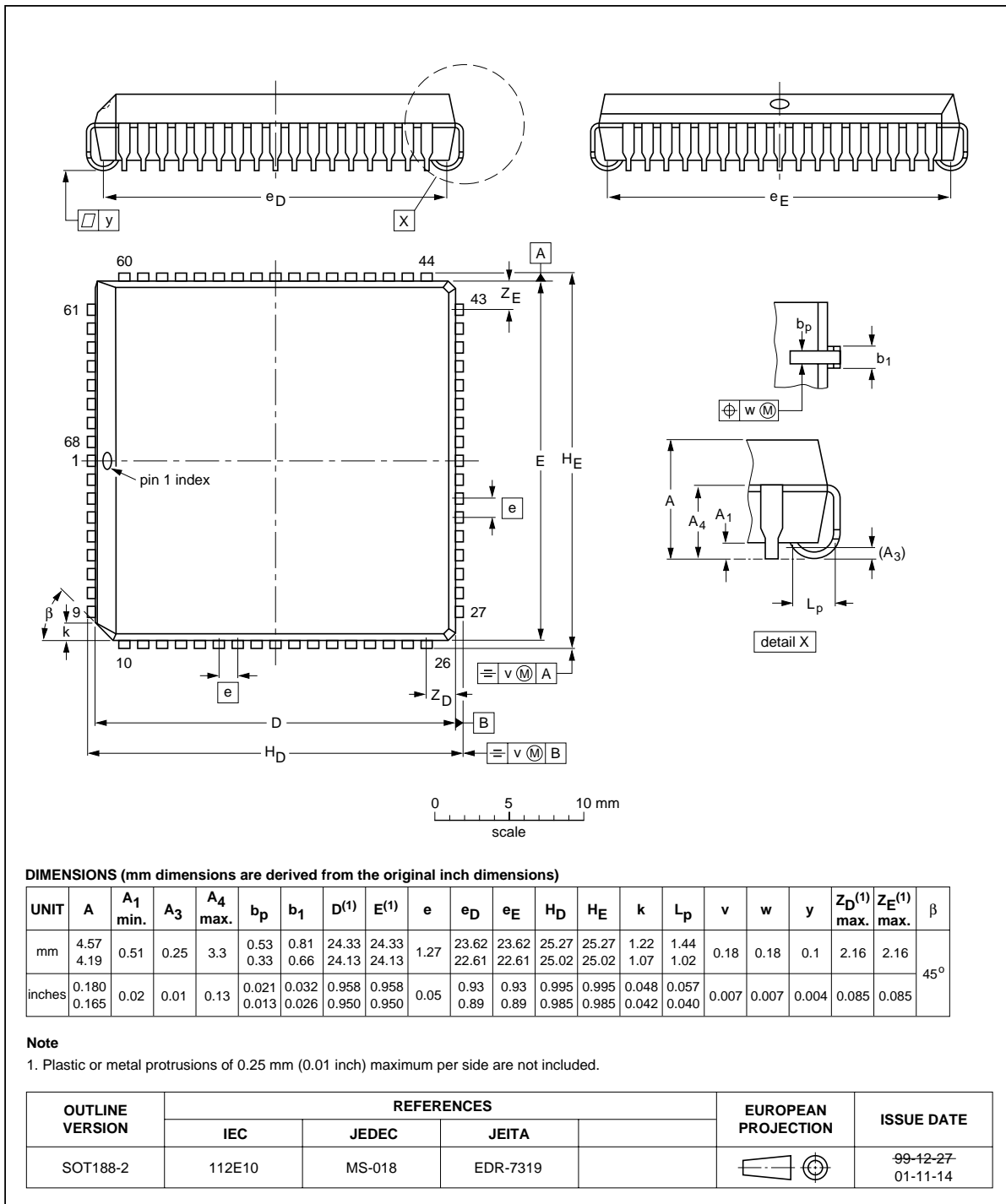
Fig 26. PLCC68 package outline (SOT188-2)
