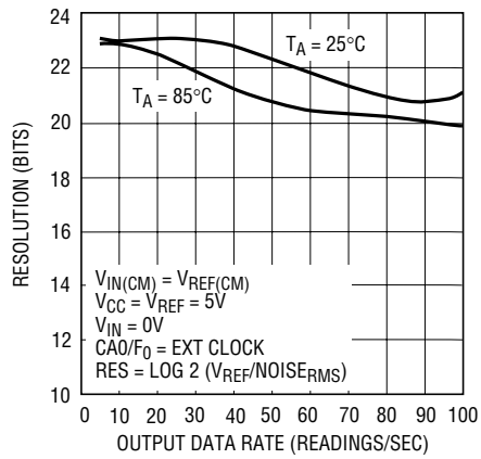
Figure 24. Resolution ( Noise_{RMS} \leq 1LSB ) vs Output Data Rate and Temperature
