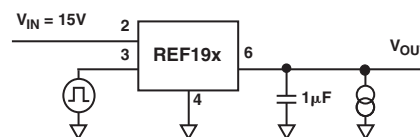
TPC 11b. \overline{\text{SLEEP}} Response Time Measurement Circuit
