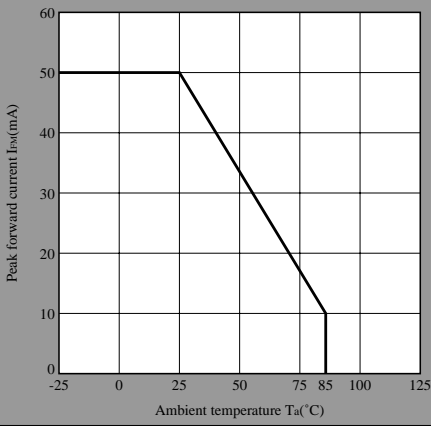
Peak Forward Current Derating Curve
