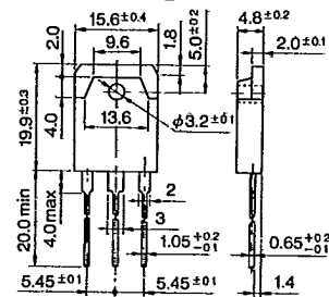
Outline Drawing ⑨
