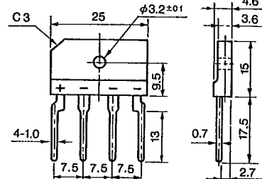
Outline Drawing ⑫
