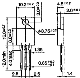
Outline Drawing ⑥⑧
