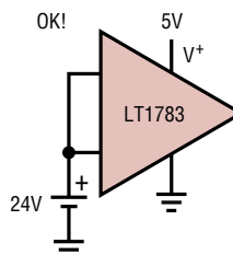
INPUT OVERVOLTAGE
