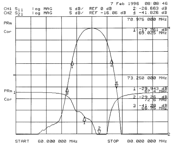
Figure 1: Frequency Response
