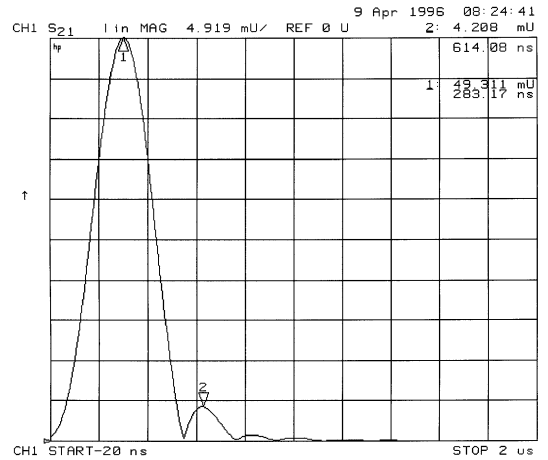
Figure 2: Impulse Response
