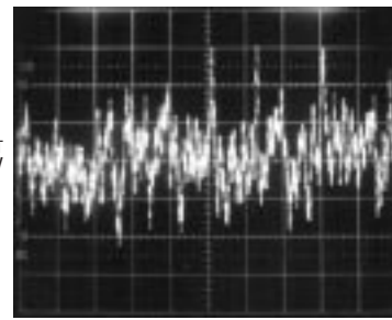
LT1761-5 10Hz to 100kHz Output Noise C_{\text{BYP}} = 100\text{pF}
