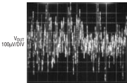
LT1761-5 10Hz to 100kHz Output Noise C_{\text{BYP}} = 0
