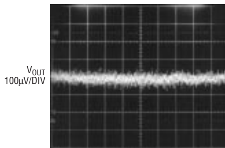
LT1761-5 10Hz to 100kHz Output Noise C_{\text{BYP}} = 0.01\mu\text{F}
