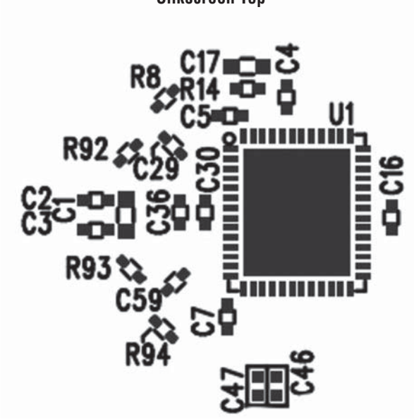
Silkscreen Top
