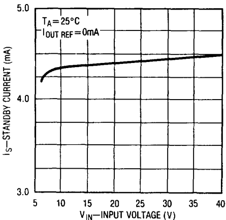
Standby Current
