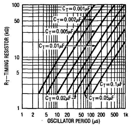
Oscillator Period
