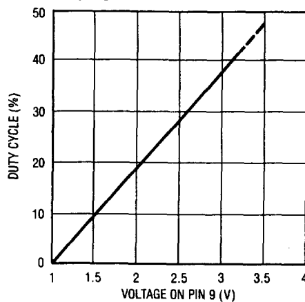
Duty Cycle
