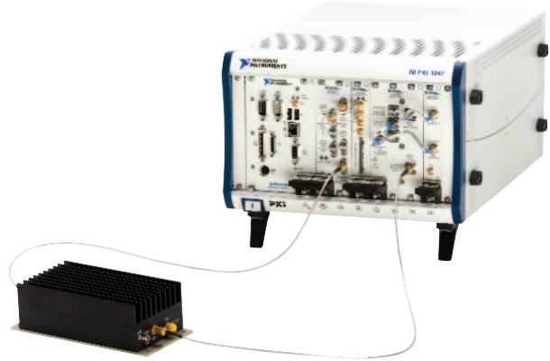
Figure 3. RF test system – PXI-5670 and PXI-5660
